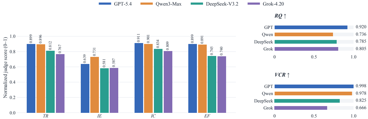
Figure 3 Tool-use capability components across four models. Left: Judge scores produced by Qwen3.5-397B-A17B over 170 traces per evaluated backbone: Tool Relevance (TR), Invocation Efficiency (IE), Information Coverage (IC), and Evidence Faithfulness (EF). Right: Routing Quality (RQ) and Valid Call Rate (VCR). All scores are shown on a 0–1 scale, with higher values indicating better performance. Hallucination-Free Rate (HFR) is omitted because all four models score 1. Additional judge results and complete metrics are provided in Appendix C.3.
