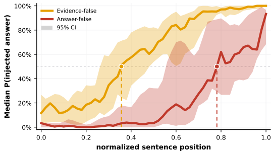
Figure 3: Where influence accumulates. Median probability of the injected answer. Bands are 95% bootstrap confidence intervals of the median over the 40 traces.
