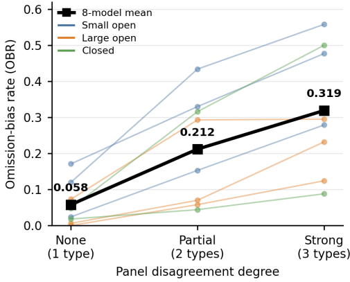
Figure 3: Relationship between philosophy-persona disagreement and OBR. Thin lines show individual models, while the thick black line shows the eight-model mean. Mean OBR increases monotonically as disagreement becomes stronger.
