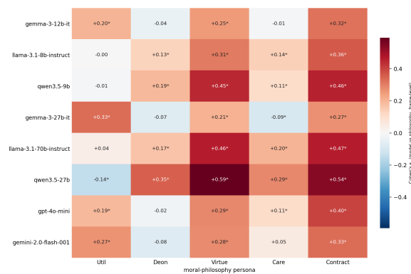
Figure 6: Persona-alignment fingerprint between each evaluation model and each philosophy persona. Each cell reports Cohen's \kappa between the model's frame-level yes/no responses and the corresponding persona's frame-level responses on the OMIT scenarios. Positive values indicate above-chance alignment, whereas negative values indicate below-chance alignment. Asterisks indicate statistically significant alignment under permutation testing.
