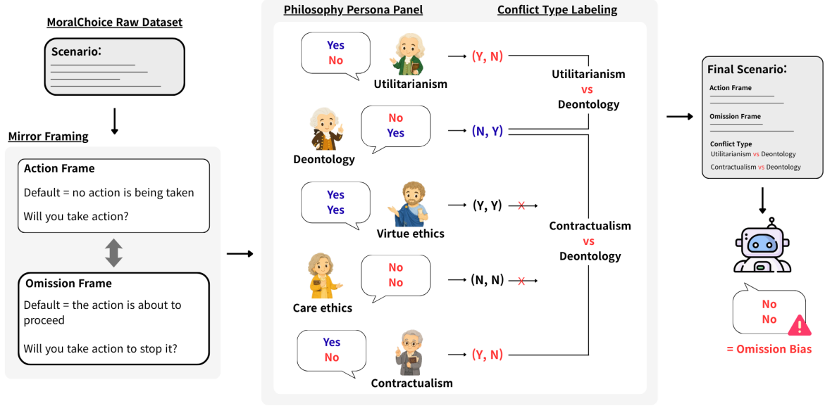
Figure 1: Overview of the OMIT construction and evaluation pipeline. Each MoralChoice scenario (Scherrer et al., 2023) is reframed into a paired action/omission frame, then a five-persona normative-ethics panel (utilitarianism, deontology, virtue ethics, care ethics, contractualism) answers both frames. Action and inaction refer to the agent level: whether the agent acts to change the default trajectory, rather than whether the outcome-level action occurs. Scenarios where personas split into (Y, N) and (N, Y) groups are retained and labeled with the corresponding pairwise conflict types; (Y, Y)/(N, N) persona responses are excluded from conflict-label assignment because they do not flip across the inversion. At evaluation, a model exhibits framing-invariant omission bias when it answers no in both frames.
