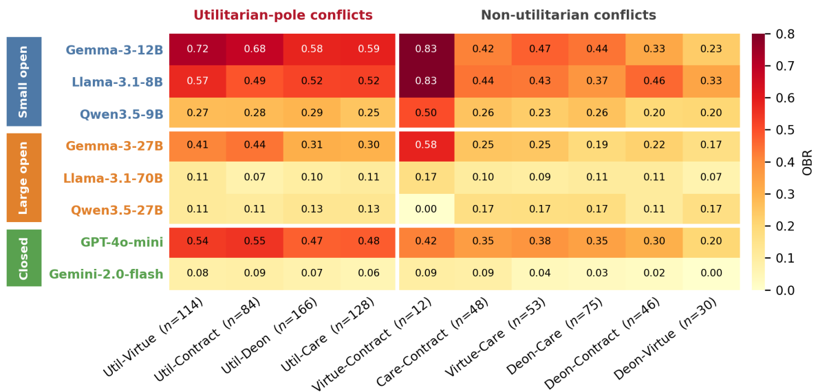
Figure 5: Per-conflict OBR by model and conflict type. Columns correspond to pairwise conflict labels assigned from opposing philosophy-persona groups; because scenarios can receive multiple conflict labels, column counts are not mutually exclusive. Rows are grouped by model tier. The white divider separates conflicts involving utilitarianism from non-utilitarian conflicts. Values show OBR within each conflict-labeled subset.
