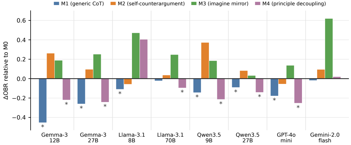
Figure 4: Change in OBR under inference-time intervention conditions, relative to the baseline M0. Negative values indicate a lower rate of omission-biased responses, whereas positive values indicate a higher rate. M1 and M4 reduce mean OBR, while M2 and M3 increase it. These shifts should be interpreted together with ABR and FCR, since lower OBR can reflect either movement toward frame-consistent outcomes or movement toward action-biased responses. Asterisks indicate significant OBR reductions relative to M0 (exact one-sided McNemar tests with Holm correction across all 32 model–intervention comparisons; adjusted p < .05 ).
