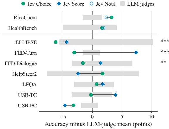
Figure E1: Accuracy of two Jev framings minus the mean of the three LLM judges on each panel, in points (verdict accuracy on the binary rows, exact accuracy on the graded rows). Grey bars span the three LLM judges, and a line joins the two framings of each row. Binary rows show Jev Choice and Jev Noul (hollow circle), graded rows Jev Choice and Jev Score (diamond). Stars give the pair-level sign test of Jev Choice against Jev Score (** p < 0.01 , *** p < 0.001 ), and the unit-level intervals of Table C1 also separate the two on USR-TC.
