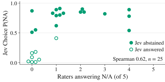
Figure F1: FED-Dialogue error_recovery: Jev Choice’s probability on the NA option for each of the 25 sampled dialogues, against the number of its five crowd workers who answered N/A, with markers of equal count spread sideways. Filled markers are the 17 dialogues on which Jev Choice abstained and hollow markers the 8 it answered (Spearman \rho = 0.62 between the probability and the number of N/A answers).
