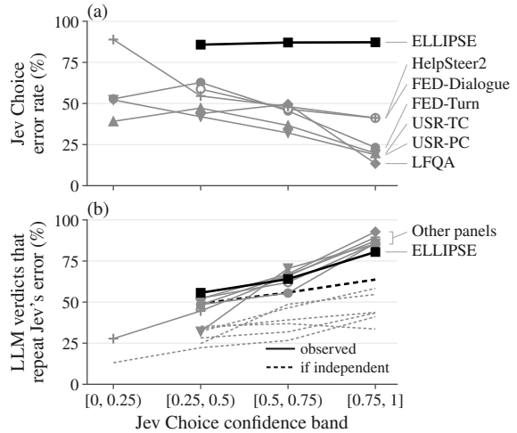
Figure 4: Jev Choice’s confidence band against (a) its error rate and (b) the share of the three LLM judges’ verdicts on its wrong pairs that repeat its wrong answer (solid), with the independence baseline of Section 6.2 (dashed). One line per graded panel, ELLIPSE in black and the other six panels in grey. Bands with fewer than 20 pairs (a) or 20 Jev errors (b) are omitted.
