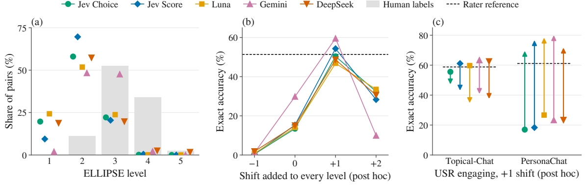
Figure 3: (a) Share of ELLIPSE pairs at each level for the human labels (grey bars) and five judges (markers, with DeepSeek over the 1,543 pairs it answered). (b) ELLIPSE exact accuracy after a post-hoc shift that adds a constant s to every predicted level, clipped to the scale, with the rater reference dashed. (c) USR engaging: exact accuracy before (marker) and after (arrowhead) a post-hoc shift of +1 level, with dashed segments at each corpus’s unshifted rater reference on engaging alone (58.8% on Topical-Chat and 61.1% on PersonaChat, below the panel-level values of Table 2); Section 5.4 compares the shifted judges with a shifted rater.
