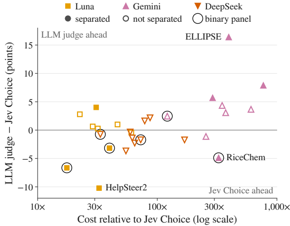
Figure 1: Paired accuracy difference in points (LLM judge minus Jev Choice of Section 3.1, over the pairs both judges scored) against the LLM judge’s cost relative to Jev Choice on the same panel, one marker per judge and panel. Filled markers are separated comparisons (Section 3.5; Table C1 gives every interval). Ringed markers are the two binary panels.
