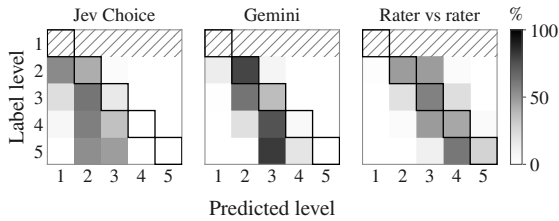
Figure G1: Row-normalized ELLIPSE confusion matrices for Jev Choice, Gemini, and one rater against the other, with the diagonal outlined. Rows are the label level and columns the predicted level. For the raters, rows are one rating and columns the other rating of the same essay and trait, with both orders pooled. The level-1 rows hold fewer than 20 pairs and are omitted (hatched).
