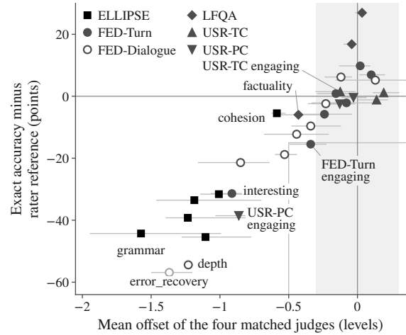
Figure 2: Mean offset of the four matched judges (whiskers: their range) against their mean gap (Section 3.5), for each of the 31 criteria that have a rater reference. Marker shape gives the panel, the shaded band marks absolute offsets below 0.3 levels, and the grey guide bounds the region with a mean offset above -0.5 levels and a gap below -15 points, which holds only FED-Turn engaging. FED-Dialogue error_recovery, whose label averages one to five raters, is drawn in light grey.
