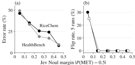
Figure D1: Jev Noul on RiceChem (black) and HealthBench (grey). (a) Error rate by the margin |P(\text{MET}) - 0.5| in five bands of 0.1, on the full RiceChem set (8,392 pairs) and on HealthBench (406 pairs). (b) Share of pairs whose verdict changed across five runs, by the same bands, on the RiceChem panel (819 pairs) and a 59-pair HealthBench subset, with hollow markers for bands of fewer than 20 pairs.
