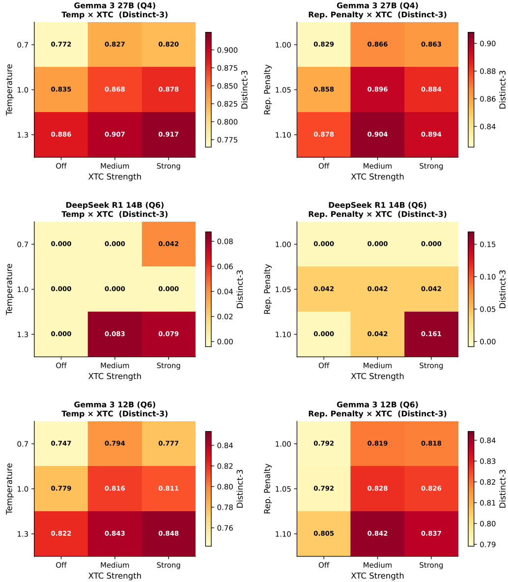
Figure 24: Interaction heatmaps: Distinct-3 surface over the temperature × XTC grid and the repetition penalty × XTC grid for each of the three model families. Diagonal structure (improvement increasing along both axes independently) is consistent with additive composition.
