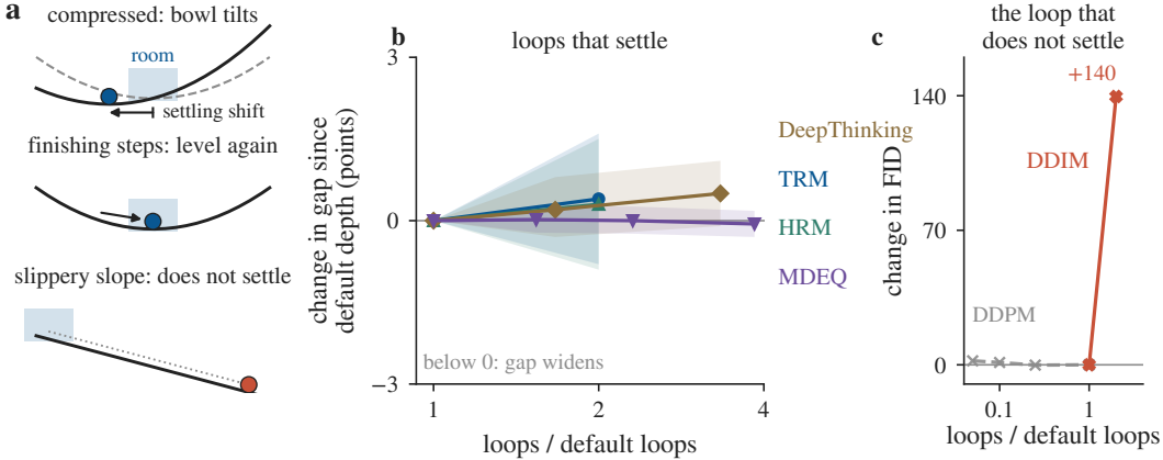
Figure 1: Thinking longer does not hurt a compressed model whose loop settles; a loop that does not settle piles up error. (a) Compression tilts the bowl, so the loop settles slightly off target. The answer survives while the settling shift stays within the room, and finishing steps level the bowl again. On a slippery slope, every loop carries the ball further. (b) Change in the gap between a 4-bit model and its own full precision as the loops go on past the default depth, one model per family; a value below zero means the gap widens. No interval lies below zero. (c) DDIM, the one loop that does not settle, adds 140 FID over the same range. Paired 95% intervals; the looped language models are in Table 2; protocol in App. C.
