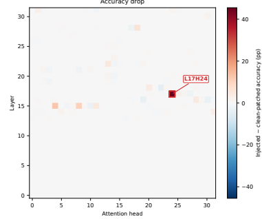
Figure 4: Individual-head patching in LLaMA-3.1-8B-IT. Reduction in correct-position accuracy, \Delta_h , in percentage points for each head.
