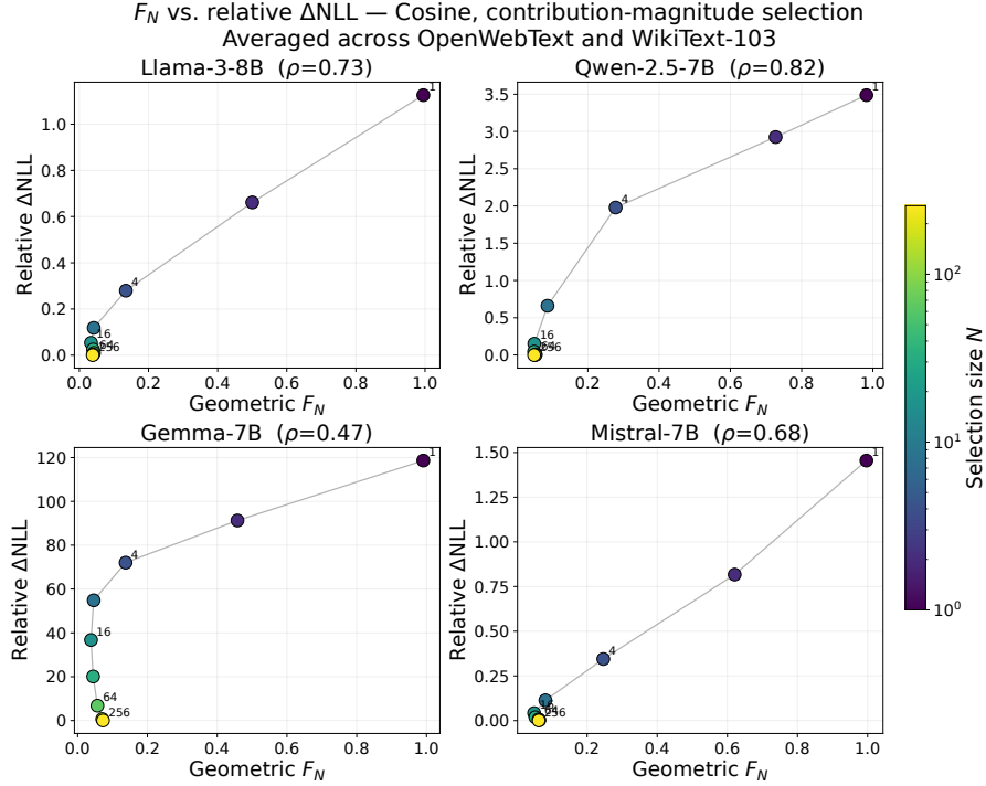
Figure 12: Contribution ranking gives similar geometry–loss trajectories. Each point corresponds to a selected-set size N , with geometric F_N and relative NLL degradation averaged across OpenWebText and WikiText-103. Color denotes N , lines connect successive sizes, and \rho is the Spearman correlation along each trajectory. Geometry is measured at the final query, while loss uses interventions throughout the model.
