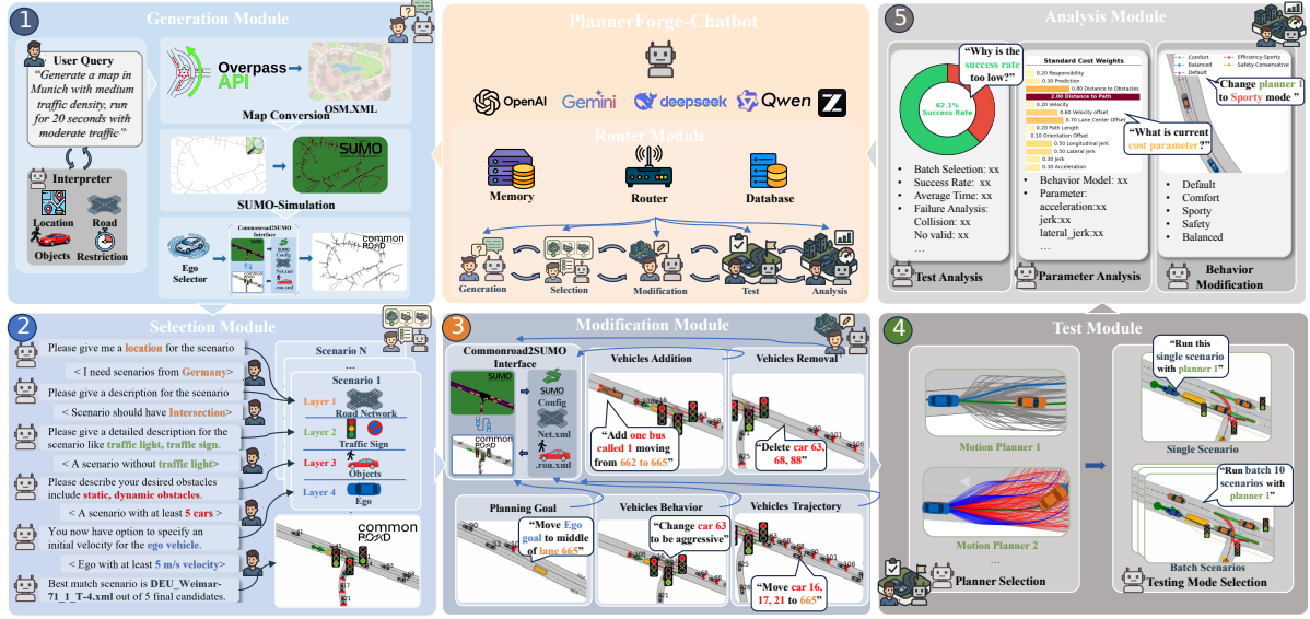
Figure 2: PlannerForge framework with six modules: Router (classifies user intent post-selection), Generation (OSM+SUMO synthesis), Selection (dialogue-guided retrieval from the CommonRoad DB), Modification (LLM-guided SUMO edits), Testing (Frenetix / MP-RBFN execution), and Analysis (LLM-powered result interpretation).
