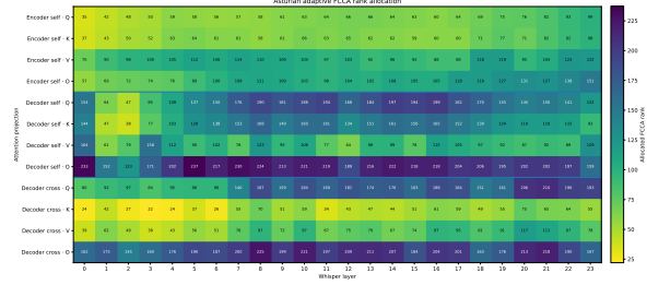
Fig. 1: Adaptive FCCA rank allocation across Whisper model layers and attention projections for Asturian. Darker cells indicate larger allocated rank.
