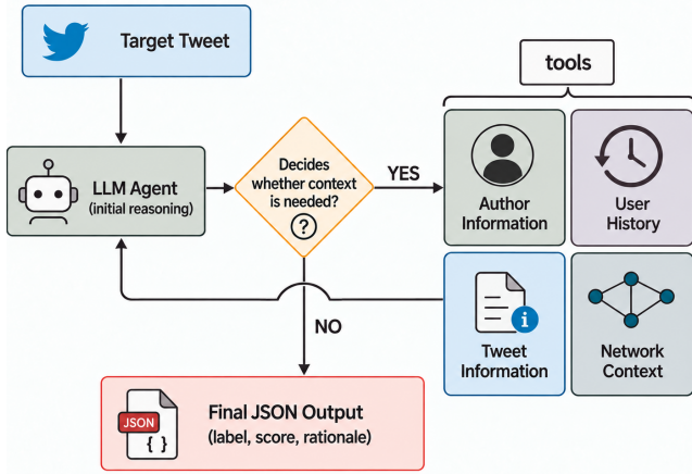
Figure 1: Full agentic workflow.
