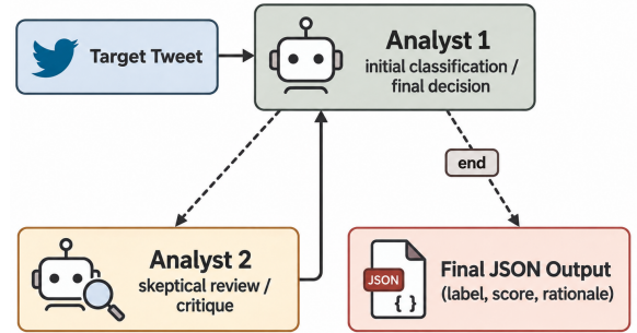
Figure 2: Two-agent debate workflow. Analyst 2 critiques Analyst 1’s initial decision before the final prediction.
