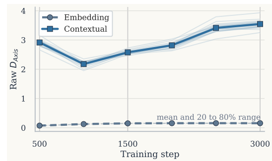
Figure 6: Dense checkpoints show an early, persistent hidden-state gap. Lines average all eight Equal exposure + shared data families at 500-step intervals; shaded bands show the 20 to 80% language range.
