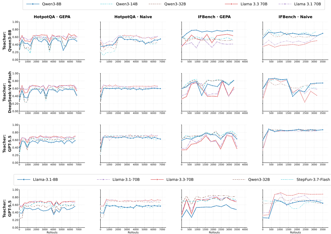
Figure 8: Optimization trajectories for the cross-student transfer experiments. Columns correspond to dataset–optimization-method combinations; rows correspond to teacher models.
