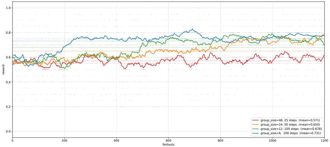
Fig. 10. GRPO training performance under different rollout group sizes.
