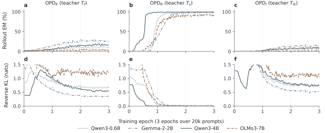
Figure 5: Training curves for on-policy distillation in the synthetic experiments. Columns correspond to distillation from T_f (a, d), T_s (b, e), and the joint T_{fs} (c, f). Top row: exact-match accuracy of sampled student rollouts on the distillation prompts; bottom row: reverse KL in nats. All runs train for three epochs over 20,000 prompts.
