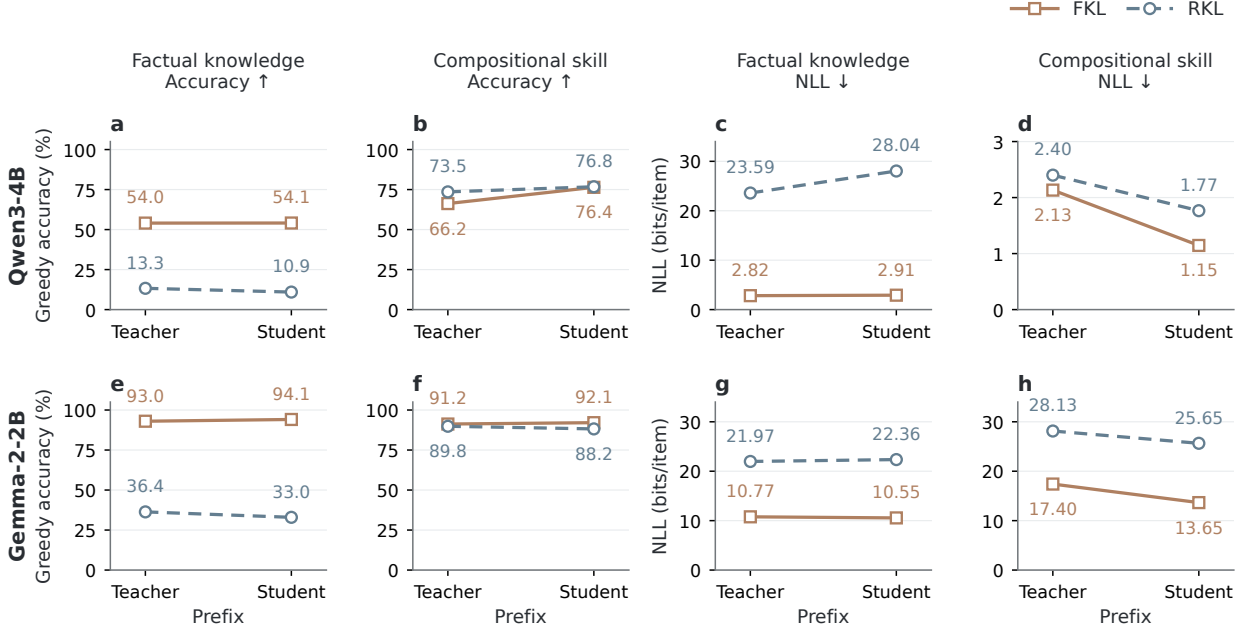
Figure 3: Effects of prefix source and KL direction. Rows show Qwen3-4B and Gemma-2-2B. Factual knowledge is evaluated after distillation from T_f ; compositional skill after distillation from T_s . Accuracy measures greedy final answers; NLL is reported for reference completions in bits per completion. Reference prefixes come from teacher demonstrations.
