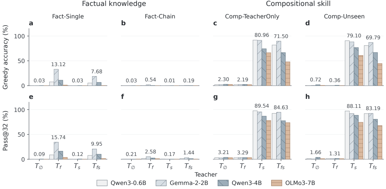
Figure 2: Student performance after on-policy distillation under each teacher. Top: greedy final-answer accuracy; bottom: final-answer Pass@32 (at least one of 32 sampled completions correct). Numbers above each group show the unweighted mean across four models. All values are percentages.
