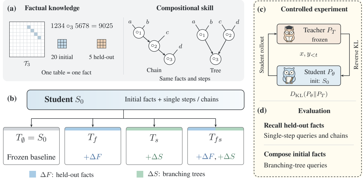
Figure 1: Overview of the setup. (a) Random lookup tables represent facts; chains and trees specify how their query results are combined. (b) Starting from S_0 , teachers add exposure to held-out facts ( \Delta F ), branching trees ( \Delta S ), or both, with frozen S_0 as the baseline. (c) A fixed teacher supervises student rollouts with reverse KL. (d) Evaluation separates factual recall on held-out facts from compositional skill over initial facts.
