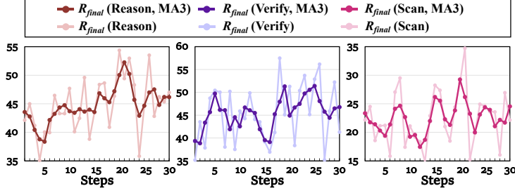
Figure 3: Left: Training dynamics of main experiments. Right: Metrics change after VERA-RL on Scan (test set).
