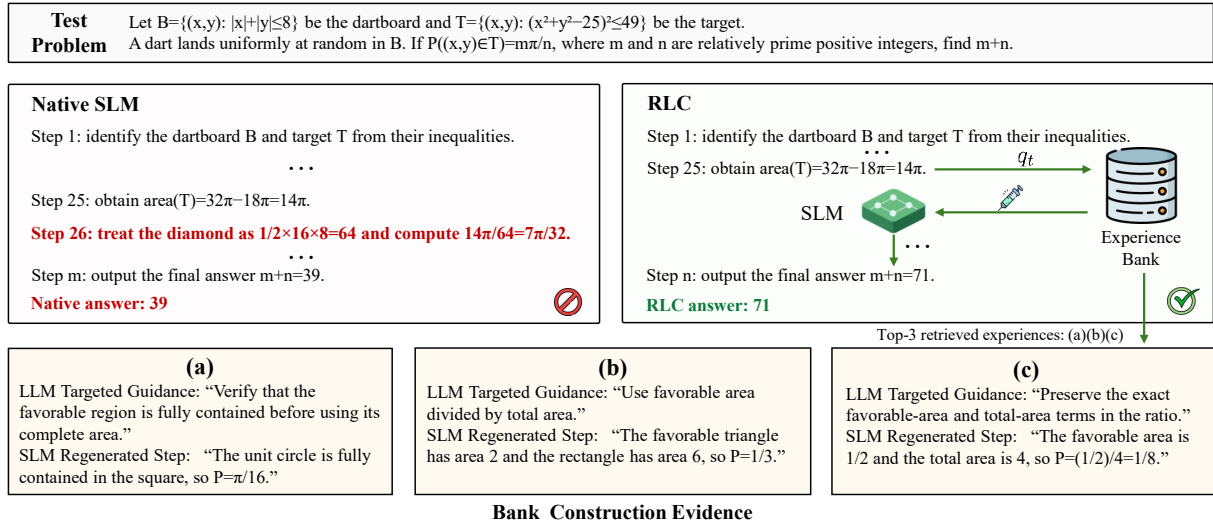
Figure 8: Case study of online latent experience reuse on AMC24. RLC retrieves relevant latent Bank entries to correct a local reasoning error and steer the frozen SLM toward the correct solution. The displayed Bank Construction Evidence is provided only to interpret the retrieved latent experiences and is not used during online inference.
