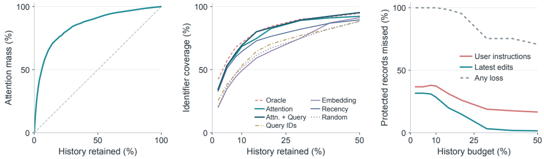
Figure 6: Additional historical-context observations. Left: Aggregate attention concentration under a retained-history budget; the diagonal denotes uniform attention per unit of history. Mid- dle: The full comparison of selection signals, including query identifiers and query embeddings. Right: User-instruction and latest-edit records omitted by attention-ranked selection, together with the fraction of transitions losing any protected record. The selector receives enough budget to fit the complete protected set.
