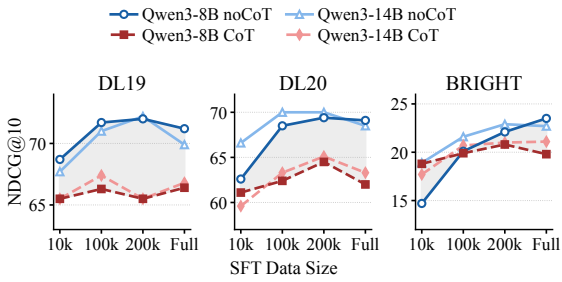
Figure 1: Performance gap between Pointwise CoT and direct scoring (noCoT) across data scales on Qwen3. The Qwen2.5 results are provided in the Appendix D.
