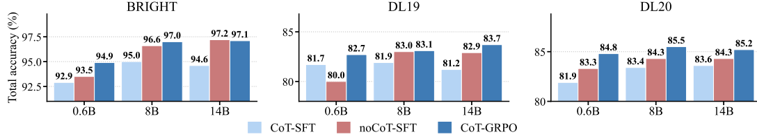
Figure 2: Total classification accuracy (%) of Qwen3 across scales: GRPO matches noCoT in 8/9 cells, yet NDCG@10 still trails (Table 2).
