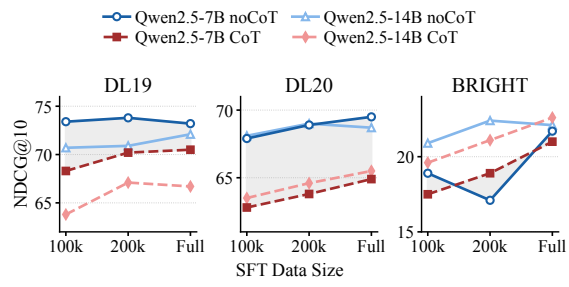
Figure 3: Data scaling on Qwen2.5 series.
