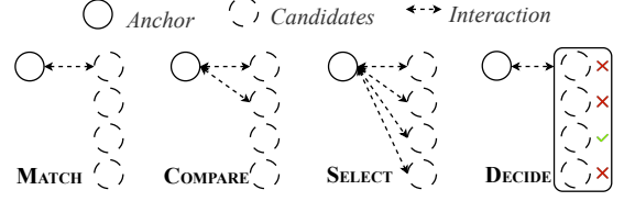
Figure 2: Interaction patterns of the operators used in CaRL-EM: MATCH , COMPARE , SELECT , and DECIDE .
