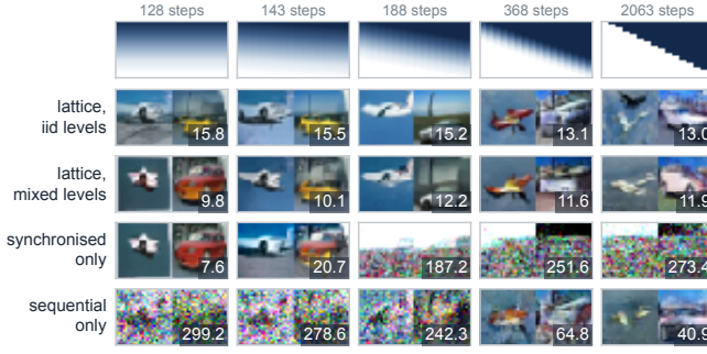
Figure 2: Both corners from one weight set. Pixels: columns give schedules and step counts (Figure 1), rows give training distributions, and cells show 2 samples and CIFAR-10 FID-50K. Tokens: text8 bpc at 85M; AR-chain rows use the identity order and masked-ELBO rows the masked-diffusion bound (protocol in Appendix B.2).
