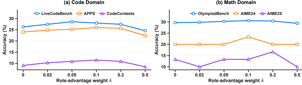
Figure 6: Accuracy of MAS-OPD as a function of the role-advantage weight \lambda . Each panel reports the three benchmarks of one domain for the 1.7B student, trained once per setting rather than repeated over seeds, so the settings \lambda = 0 and \lambda = 0.1 are single-run instances of the w/o RAS and MAS-OPD systems of Table 2 rather than the five-run averages given there. The two AIME sets contain thirty problems each, where one problem is worth 3.3 points, which is why those curves move in larger steps than the other four. The two panels share a common vertical span so that the dependence on \lambda can be compared between the domains.
