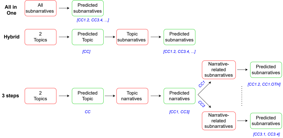
Figure 1: Overview of the three SemEval classification schemes.
