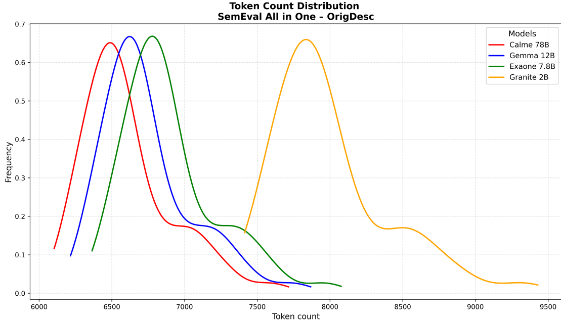
Figure 7: Distribution of the number of input tokens per document for the OrigDesc prompt strategy on the SemEval dataset across the four evaluated models.
