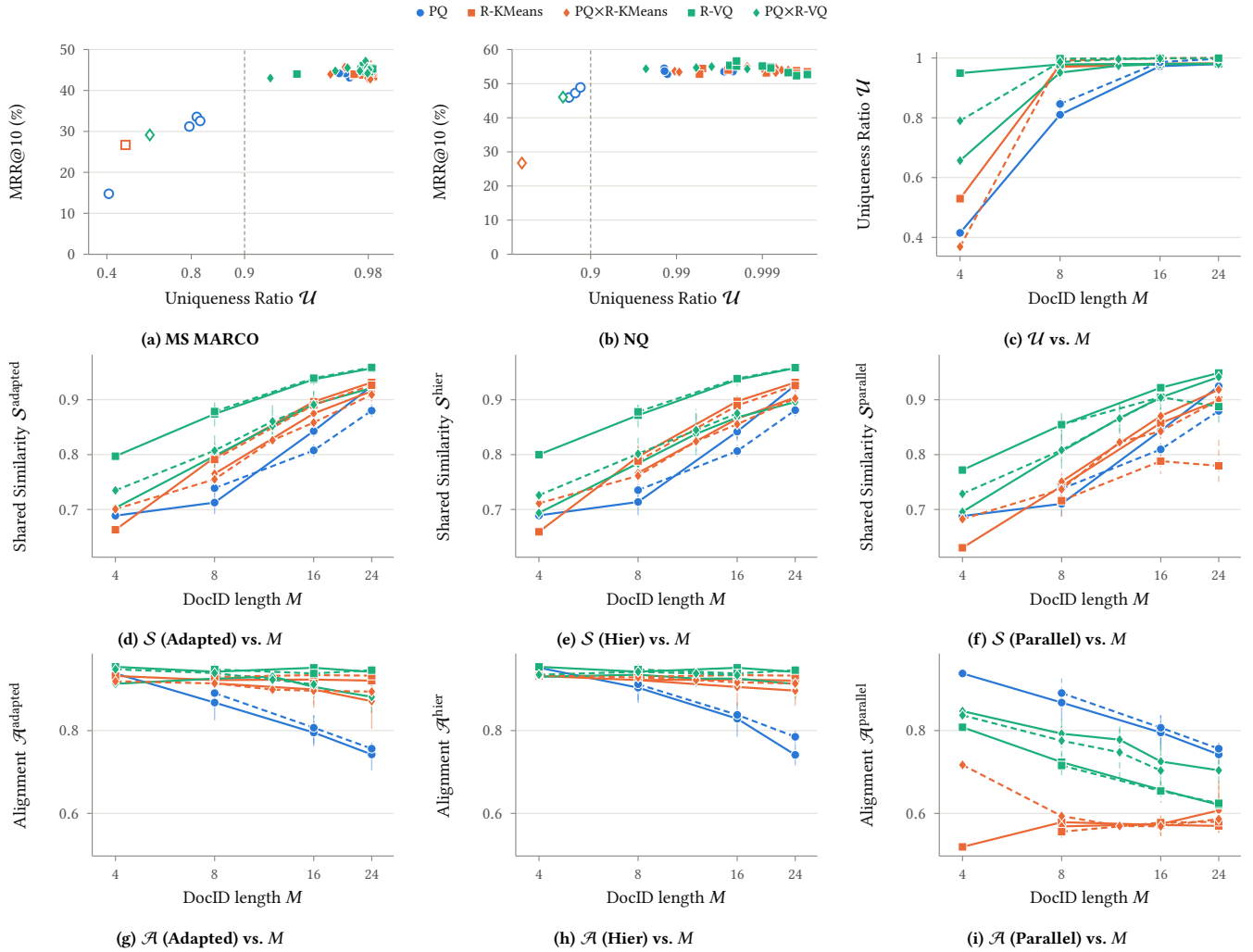
Figure 3. Uniqueness Ratio \mathcal{U} , Shared Semantic Similarity \mathcal{S} and Contrastive Alignment Preservation \mathcal{A} . (a) and (b) Uniqueness \mathcal{U} vs. MRR@10 on MS MARCO and NQ, one marker per configuration (color and shape: family), hollow: \mathcal{U} < 0.9 , measured or implied by V^M < 0.9N (at most V^M distinct DocIDs); \mathcal{U} axis stretched toward 1 (log scale of the collision rate), dashed line: \mathcal{U} = 0.9 . R^2 of MRR@10 on the metric, MS MARCO / NQ: \mathcal{U} 0.94 / 0.97. (c) to (i): Impact of DocID length M and evaluation formulation on Uniqueness ( \mathcal{U} ), Shared Similarity ( \mathcal{S} ) and Alignment ( \mathcal{A} ) MS MARCO: full lines, NQ: dashed lines. (d) to (f): \mathcal{S} , (g) to (i): \mathcal{A} , in their Adapted (Section 3.2.2), Hier and Full variants
