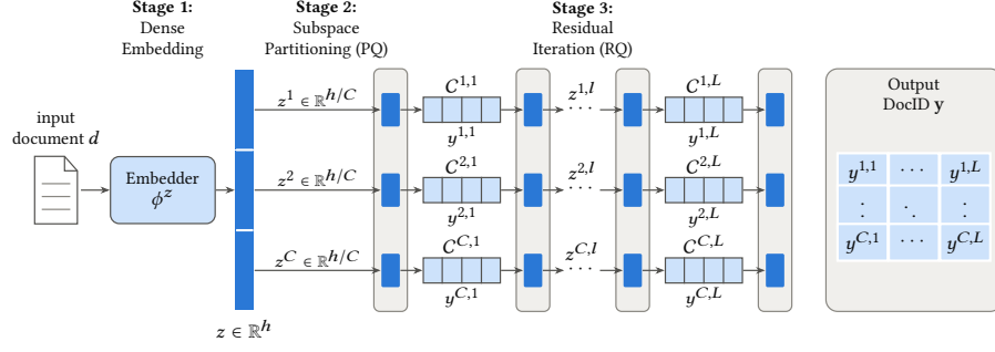
Figure 1. Unified framework for semantic DocID encoding. Stage 1: the embedder \phi^z maps a document d to a dense vector z . Stage 2 splits z into C sub-vectors z^c (PQ, C > 1 ). Stage 3 quantizes each sub-vector with L residual codebooks C^{c,l} of V codewords (RQ, L > 1 ), each step emitting one token y^{c,l} of the DocID y ( M = C \times L tokens). (C, L) and the codebook training ( k -means or learned) recover PQ ( L = 1 ), R-KMeans and R-VQ ( C = 1 ), and the hybrids PQ×R-KMeans and PQ×R-VQ ( C, L > 1 ).
