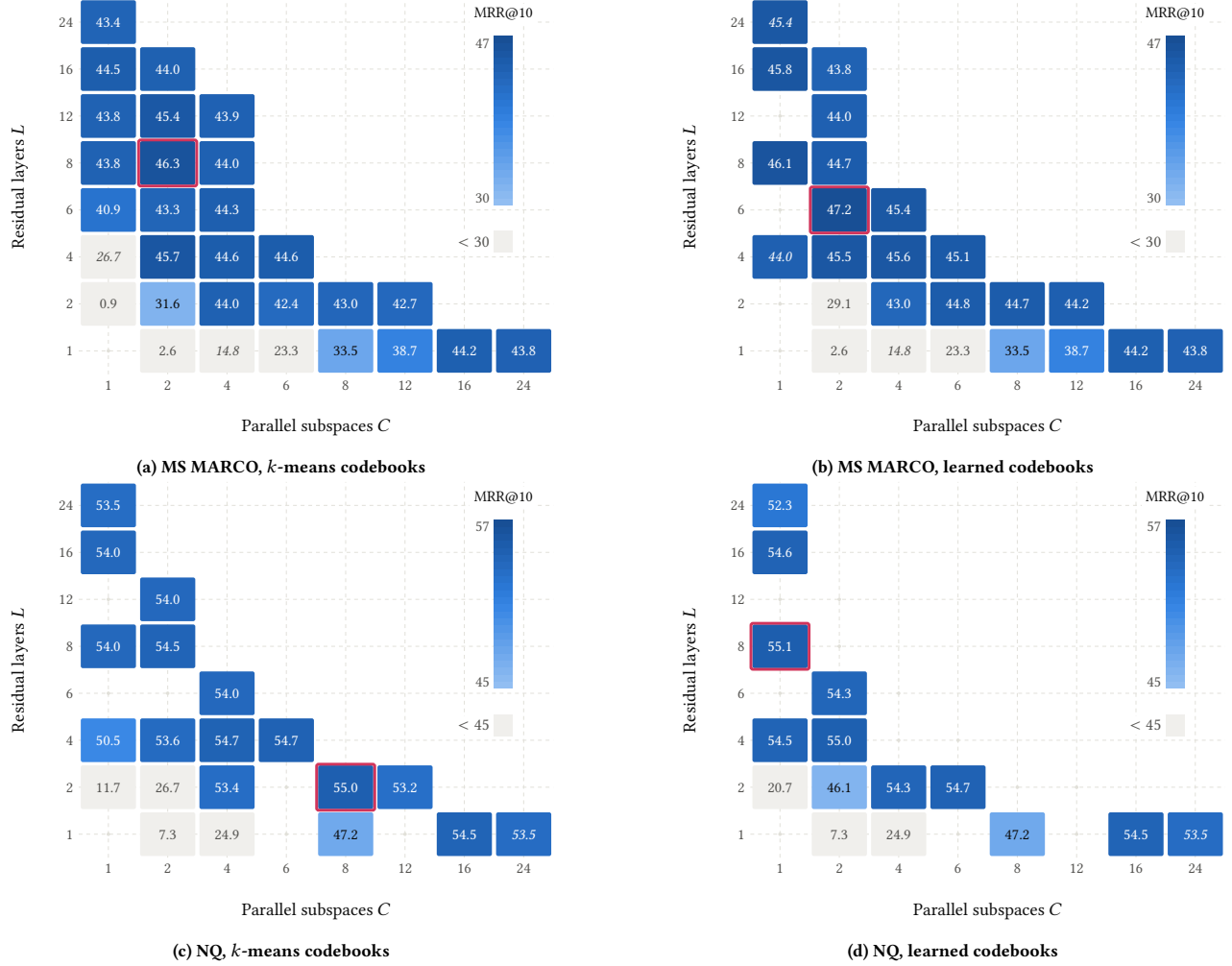
Figure 2. MRR@10 (%) over the grid of C parallel subspaces and L residual layers, with V = 256 codewords per codebook. PQ has only one training regime: its row ( L = 1 ) is the same in every panel. Red outline: best cell of the panel; pale cells lie below the color range; italics: no run at V = 256 , mean over V \in \{128, 512\} .
