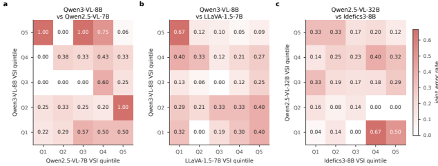
Figure 5: Joint VSI quintiles across three representative model pairs on POPE, coloured by joint error rate. The low-VSI corner concentrates joint errors; this is the visual form of the sample-intrinsic claim of §2.3.
