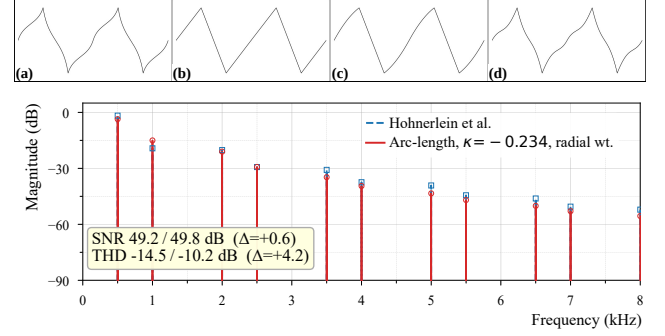
Figure 2: Triangle, N = 3 . (top) Waveforms ( f_0 = 110 Hz, f_s = 44.1 kHz): (a) angular-velocity [1], (b) arc-length, no correction, (c) \kappa = -0.234 , (d) \kappa = -0.234 with radial weighting. (bottom) Spectra of (a) (blue dashed) vs (d) (red) at f_0 = 500 Hz, f_s = 48 kHz; SNR/THD deltas inset.
