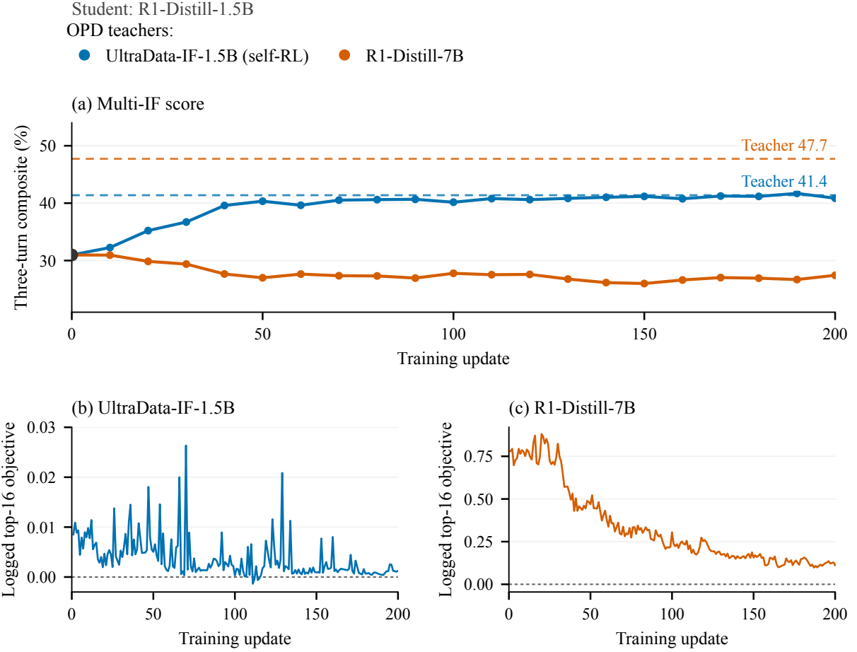
Figure 7: Instruction-following dynamics over 200 updates. (a) Three-turn composite scores; the black point is the shared initial student, and dashed lines are the corresponding standalone teachers. (b,c) Raw signed top-16 objectives, without smoothing, on separate linear axes that include zero. Colors identify the teacher used for OPD.
