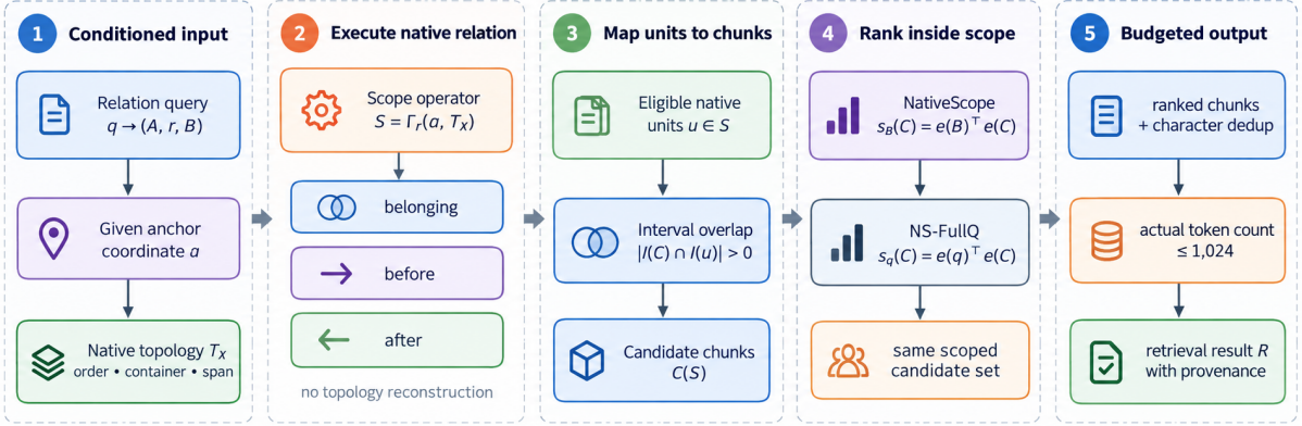
Figure 1. NativeScope pipeline
