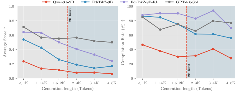
Figure 7: OOD performance on SPIQA and CharXiv combined by generation length. Average score is (\text{EA} + \text{SP} + \text{VQ})/3 . The red dashed line marks the 2K-token post-training limit.
