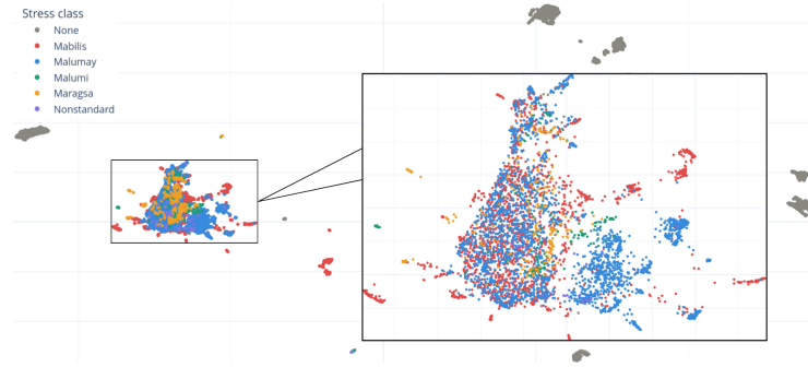
Fig. 4: UMAP word-level embeddings, colored with stress classification. Byte embeddings corresponding to one word are mean-pooled to obtain a representation for a word. Observe high degree of separation for unstressed words.
