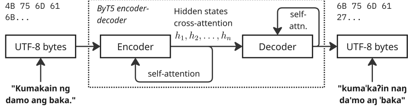
Fig. 2: Model architecture overview
