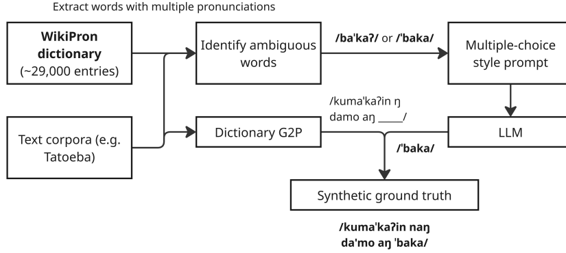
Fig. 1: Synthetic training data generation pipeline. We use the Gemini series of models as the LLM, specifically Gemini 3 Flash and 2.5 Flash Lite. In some cases, we enable the LLM’s “thinking” feature, which allows it to first generate an internal chain-of-thought loop before responding (see [25] for more information).
