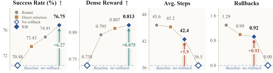
Figure 4: Where-to-recover ablation on ScienceWorld with DeepSeek-V3. No rollback retains reflection but disables state restoration; Restart restores to the initial checkpoint; Direct selection chooses a checkpoint in one stage; and RIR uses coarse-to-fine restore localization.
