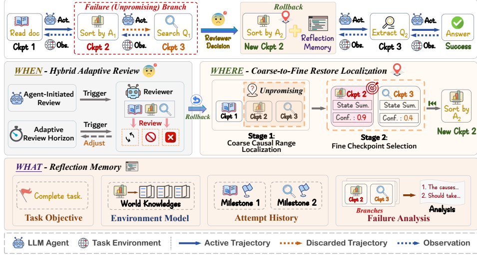
Figure 1: Overview of the Rollback-Induced Reflection (RIR) framework.
