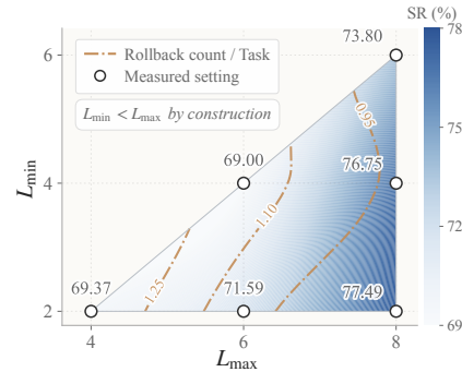
Figure 3: Sensitivity to the adaptive review range ( L_{\min} , L_{\max} ) on ScienceWorld with DeepSeek-V3. Color denotes SR and orange contours denote average rollback frequency.
