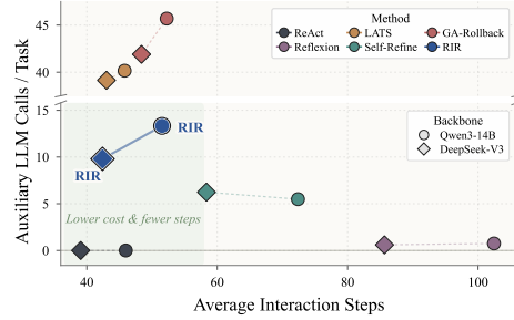
Figure 2: Efficiency trade-off on ScienceWorld across both backbones.
