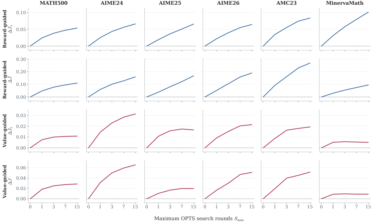
Figure F.1: Learned-critic search-budget results by benchmark. Rows report reward-guided \Delta J_{\lambda} , reward-guided \Delta J , value-guided \Delta J_{\lambda} , and value-guided \Delta J , where each difference is relative to S_{\max} = 0 . Columns show the six reasoning benchmarks.
