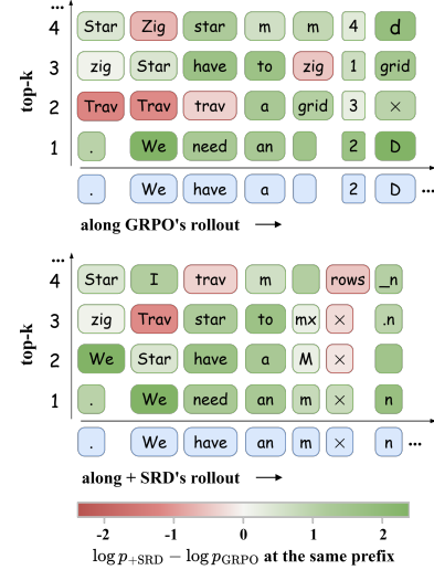
Figure 3: The same shift token by token, on one rollout per arm: rows are the top-4 likeliest continuations under the policy that owns the rollout.
