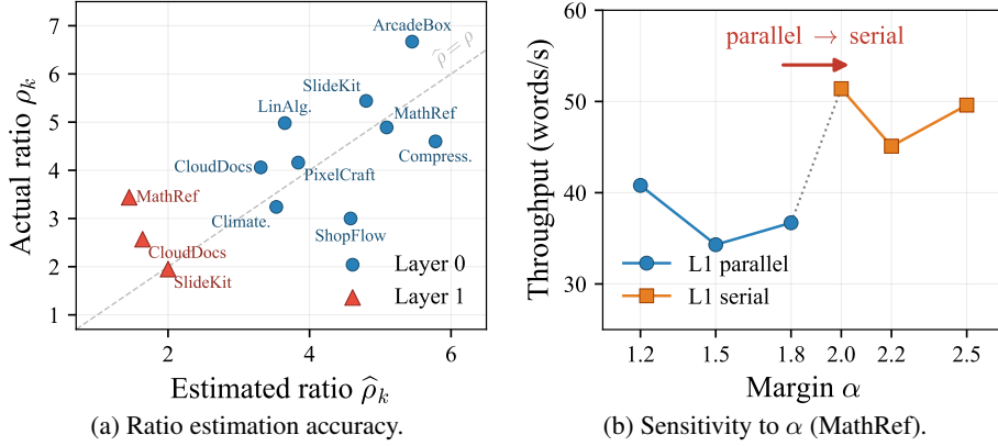
Figure 2: Scheduler sensitivity analysis. (a) Estimated cost ratio \hat{\rho}_k versus actual cost ratio measured after execution, across 14 multi-task dependency layers from 9 evaluation tasks. Layer 0 and Layer 1 correspond to the first and second dependency layers in the orchestrator-generated task DAG. (b) Throughput on MathRef under different safety margins \alpha , with the task DAG and token estimates held fixed. For \alpha \geq 2.0 , Layer 1 changes from parallel to serial execution, which improves throughput because the alignment cost of cross-referencing appendices exceeds the parallelism benefit.
