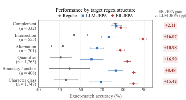
Figure 8 ER-JEPA achieves higher prediction accuracy across all six evaluated regex structures with episodic replay. Compared with LLM-JEPA, ER-JEPA improves accuracy by 16.90, 16.07, and 15.42 percentage points for expressions containing quantifiers, intersections, and character classes, respectively.
