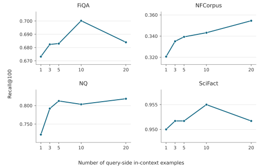
Figure 1: Recall@100 across varying numbers of in-context examples for generating RICE (Qwen3.5-9B) query encodings.
