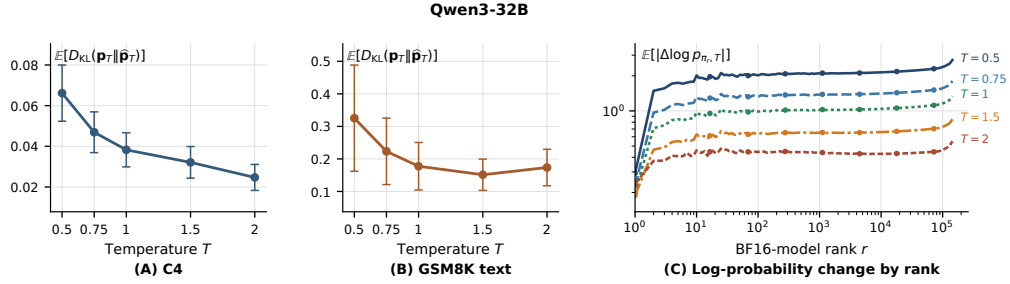
Figure 26: Next-token probability changes under temperature rescaling. (A) and (B) show the mean forward KL on C4 and GSM8K text. Error bars show standard deviation across inputs. (C) shows the actual mean absolute log-probability change over BF16-model rank for five temperatures averaged over both datasets.
