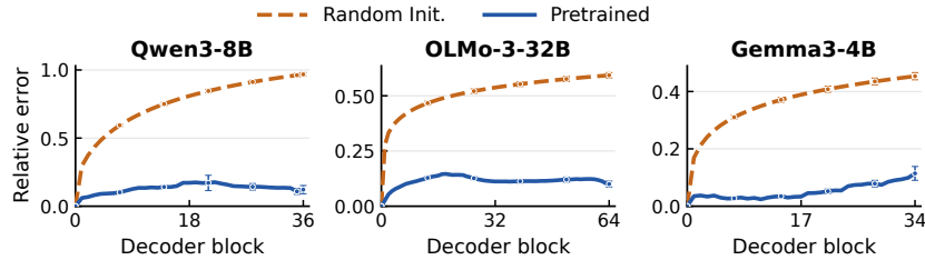
Figure 9: Randomly initialized and pretrained models across three architecture families. Relative hidden errors are shown for Qwen3-8B, OLMo3-32B, and Gemma3-4B under the same NVFP4 conversion. Error bars show standard deviation. Qwen3-8B and OLMo3-32B use BF16 for non-quantized computation; Gemma3 uses FP32 for the original pass and all non-quantized operations.
