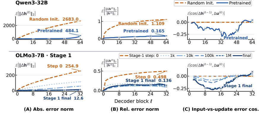
Figure 1: Pretraining changes quantized model’s hidden-error growth. Rows compare random/pretrained Qwen3-32B and OLMo3-7B Stage-1 checkpoints on C4. (A) Mean absolute hidden-error norm; (B) mean relative hidden-error norm; (C) mean cosine between the block-input error and block-update error. Error bars show standard deviation.
