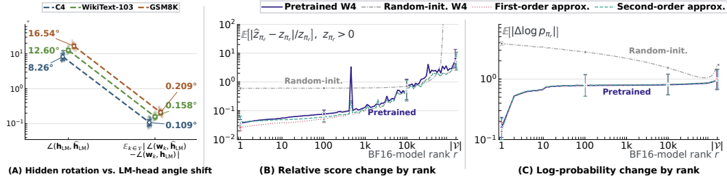
Figure 5: Top-ranked token scores and probabilities are more stable after quantization in the pretrained model. Qwen3-32B on C4, WikiText-103, and GSM8K text. (A) Across datasets, the LM-head input rotates by 8.26^\circ to 16.54^\circ , whereas the vocabulary-mean projection-angle change is only 0.109^\circ to 0.209^\circ . (B) Relative score error increases toward lower-ranked tokens and is much smaller in the pretrained model than at random initialization. The theoretical approximation is under \rho = 1 of Thm. 2. (C) Log-probability error follows the same rank trend, and the approximations follow Thm. 3. Error bars show one log-SD; details are given in App. D.3.
