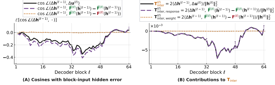
Figure 16: The response to block-input error carries counteraction in Qwen3-32B. C4 inputs. (A) Cosines between the block-input error and the block-update error \Delta \mathbf{u}^{(\ell)} , split into the direct weight effect and input-error response from Eq. (22). (B) Their contributions T_{\text{inter, weight}}^{(\ell)} and T_{\text{inter, response}}^{(\ell)} to T_{\text{inter}}^{(\ell)} . Error bars show one sample standard deviation.
