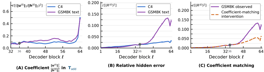
Figure 13: The update-to-hidden norm ratio explains much of the data-dependent late hidden-error growth in Qwen3-32B. (A) The coefficient \|\mathbf{u}^{(\ell)}\|_2^2/\|\mathbf{h}^{(\ell)}\|_2^2 in \mathbf{T}_{\text{add}} is larger on GSM8K text over most late blocks. (B) The relative hidden error then grows faster. (C) Matching the coefficient to the C4 values from block 36 reduces this growth. Error bars show the standard error across 64 sequences at selected blocks.
