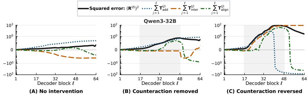
Figure 17: Relative squared-error accounting after counteraction intervention in Qwen3-32B. Columns compare unmodified W4 with counteraction removal and reversal over blocks 17–48, where counteraction is strong. The corresponding hidden-error and output changes are reported in Sec. 3.3. In contrast to the other figures, a symmetric logarithmic scale is used here to compare trajectories that span multiple orders of magnitude.
