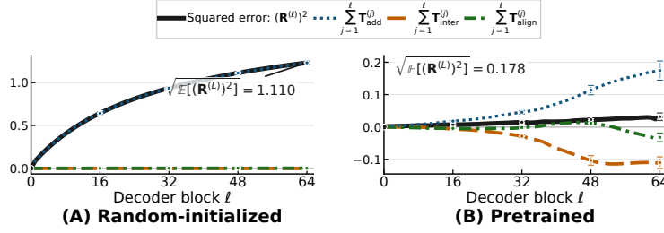
Figure 2: Accumulated contributions of the three terms in Thm. 1. Randomly initialized and pretrained Qwen3-32B on C4. Each colored curve accumulates one term over blocks 1– \ell and shows its averaged value across inputs. The black curve is their exact sum. Error bars show standard deviation across inputs.
