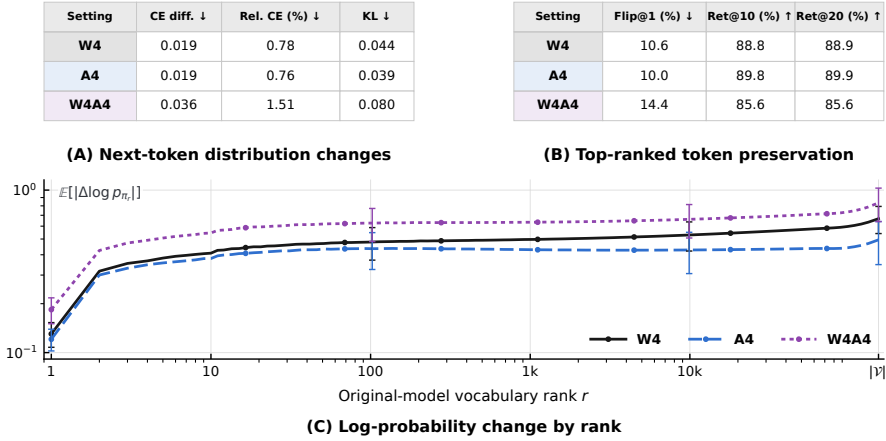
Figure 20: Output changes under weight and activation quantization. Qwen3-32B on the same C4 inputs and retained next-token positions used in Fig. 19. Metrics follow Sec. 4.1. Error bars show one sample standard deviation across complete inputs.
