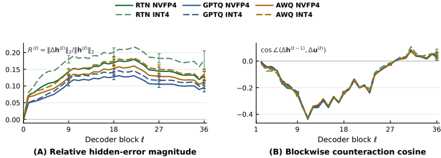
Figure 21: Counteraction is consistent across PTQ algorithms and weight formats. Qwen3-4B results. Solid and dashed curves denote NVFP4 and asymmetric INT4. Error bars show one sample standard deviation across inputs.
