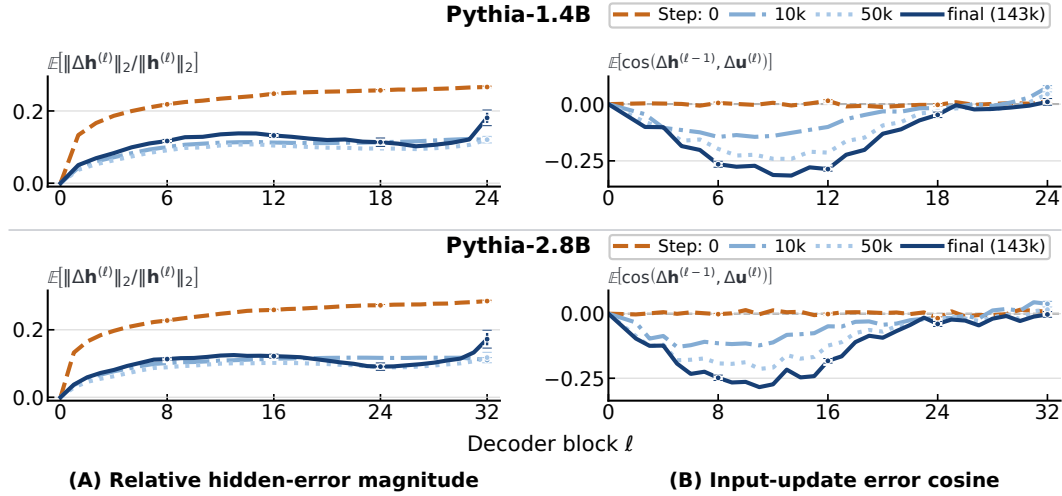
Figure 14: Counteraction strengthens during Pythia pretraining. Rows show four checkpoints of Pythia-1.4B and Pythia-2.8B under the same NVFP4 weight conversion. Columns report relative hidden error and the cosine between the block-input hidden error and block-update error. Error bars show standard deviation.
