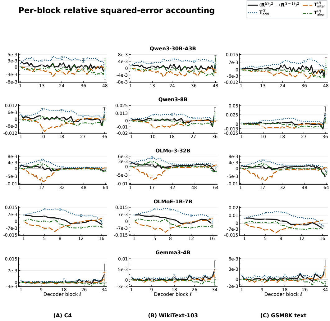
Figure 11: Per-block relative squared-error contribution. Rows are models and columns are datasets. The black curve is the exact blockwise change; the colored curves are the three terms in Thm. 1. Error bars show one sample standard deviation across complete input sequences.
