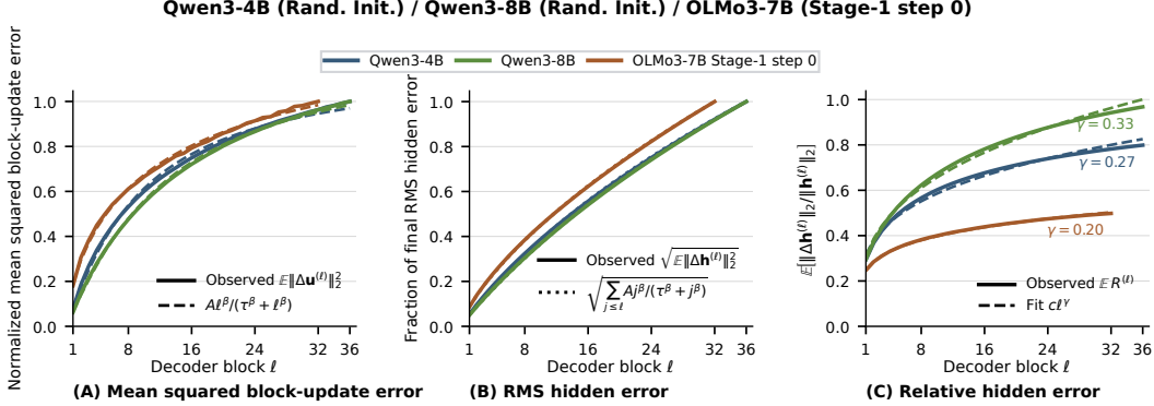
Figure 8: Fits to block-update and hidden-error growth across randomly initialized models. Results in (A) and (B) are normalized by their final values for comparison across Qwen3-4B, Qwen3-8B, and OLMo3-7B Stage-1 step 0. (A) Fitted curves follow the measured \mathbb{E}\|\Delta\mathbf{u}^{(\ell)}\|_2^2 . (B) Summing the fitted values closely matches the measured RMS hidden error. (C) Power laws fit the unnormalized mean relative hidden error. All fits are restricted to the measured blocks.
