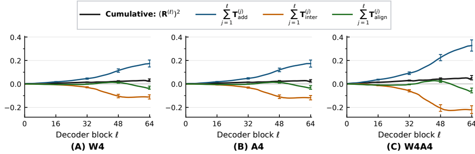
Figure 19: Relative-error recurrence under weight and activation quantization. Qwen3-32B on C4 under W4, A4, and W4A4. The black curve is the cumulative squared relative error; the colored curves are the cumulative contributions of T_{\text{add}} , T_{\text{inter}} , and T_{\text{align}} . Error bars show one sample standard deviation across complete inputs.
