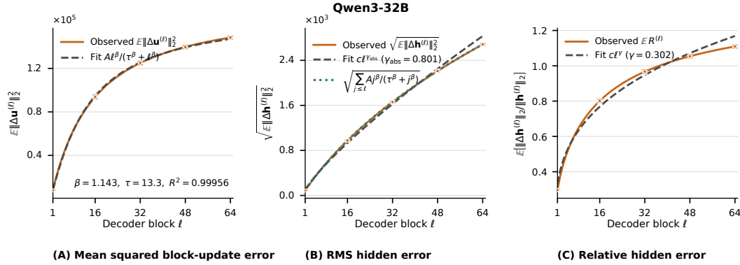
Figure 7: Fits to block-update and hidden-error growth in randomly initialized Qwen3-32B. (A) A three-parameter curve fits \mathbb{E}\|\Delta \mathbf{u}^{(\ell)}\|_2^2 over the measured blocks. (B) Summing these fitted values closely matches the measured RMS hidden error, whose growth is also fitted by a power law. (C) A separate power law fits the mean relative hidden error. Error bars show standard deviation.
