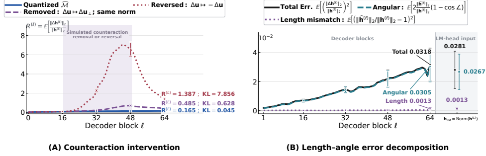
Figure 3: Counteraction interventions and length-angle decomposition of the hidden error. Qwen3-32B on C4. (A) Relative hidden error after counteraction removal or reversal. (B) Terms of Prop. 2; the separated right region shows the LM-head input terms. Error bars show SD.
