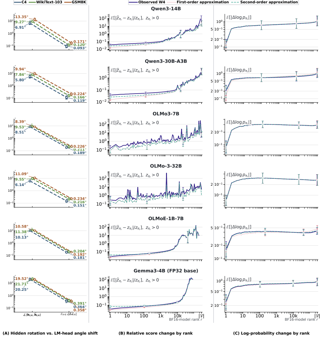
Figure 25: Top-ranked token scores and probabilities are more stable after quantization across models. Six models are evaluated on C4, WikiText-103, and GSM8K text. Projection-angle changes remain below one degree despite larger LM-head input rotations, and relative score and log-probability errors increase toward larger ranks. Score and log-probability results are averaged over the three datasets. Gemma3 uses FP32 for non-quantized computation. (B) uses the \rho = 1 approximation from Thm. 2; (C) uses the approximations from Thm. 3.
