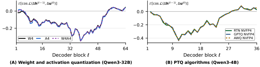
Figure 6: Blockwise counteraction across quantization components and PTQ methods. (A) Qwen3-32B on C4 under W4 (weight-only), A4 (activation-only), and W4A4 (both quantized). (B) Qwen3-4B under RTN, GPTQ, and AWQ, all quantizing the same weights with NVFP4 format.
