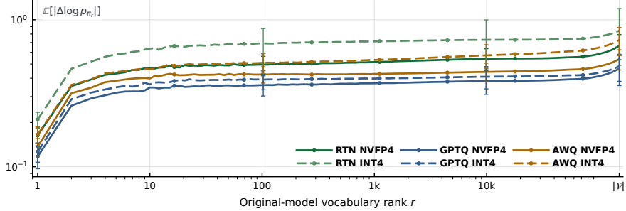
(C) Log-probability change by rank
