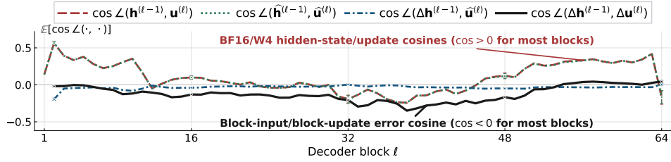
Figure 15: Counteraction is specific to the error dynamics in Qwen3-32B. BF16 and W4 hidden-state/update cosines are compared with the cosine between the block-input and block-update errors on C4 inputs. Error bars show one sample standard deviation.
