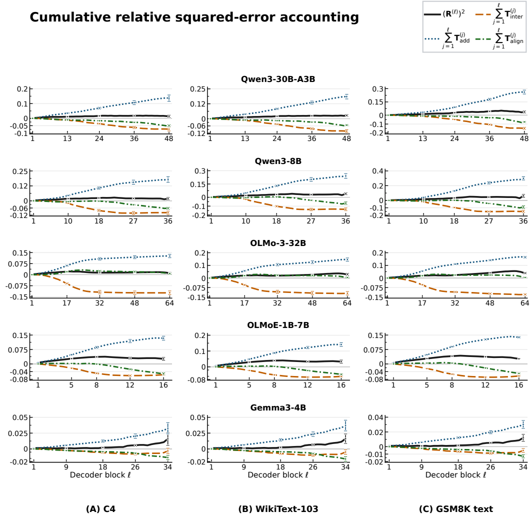
Figure 10: Cumulative relative squared-error accounting. Rows are models and columns are datasets. The black curve is the exact squared relative hidden error; the colored curves are the cumulative three-term contributions. Error bars show one sample standard deviation across complete input sequences. Position selection is described in App. E.3.
