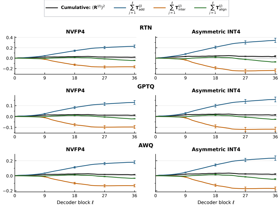
Figure 22: Relative-error recurrence across PTQ algorithms and weight formats. Qwen3-4B under RTN, GPTQ, and AWQ with NVFP4 and asymmetric INT4. Each row shows one PTQ algorithm, and the two columns share a vertical scale within that row. The black curve is the cumulative squared relative error; the colored curves are the cumulative contributions of T_{\text{add}} , T_{\text{inter}} , and T_{\text{align}} . Error bars show one sample standard deviation across inputs.
