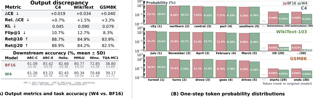
Figure 4: Output metrics and paired next-token probabilities after W4 quantization. Qwen3-32B. (A) Output-quality metrics and zero-shot benchmark accuracy. (B) Paired BF16/W4 probabilities at one representative next-token position per dataset, showing BF16 ranks 1–5 and 29–30.
