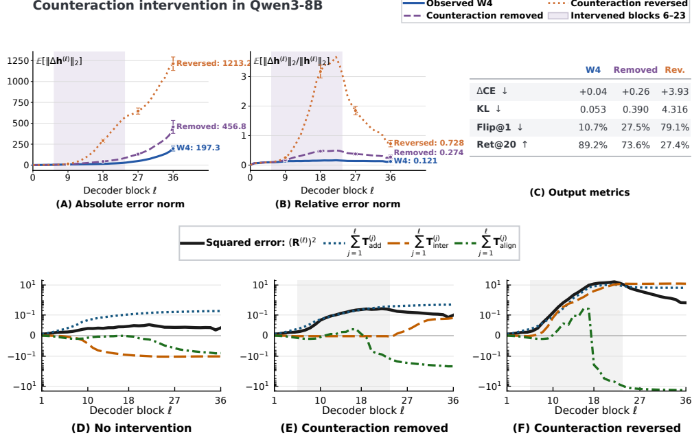
Figure 18: Counteraction intervention in Qwen3-8B. (A,B) Hidden-error trajectories and (C) output changes after removing or reversing counteraction over blocks 6–23. (D)–(F) Relative squared-error accounting along the same three trajectories. Output metrics are defined in Sec. 4.1; error bars show one sample standard deviation across inputs. The lower panels use a symmetric logarithmic scale.
