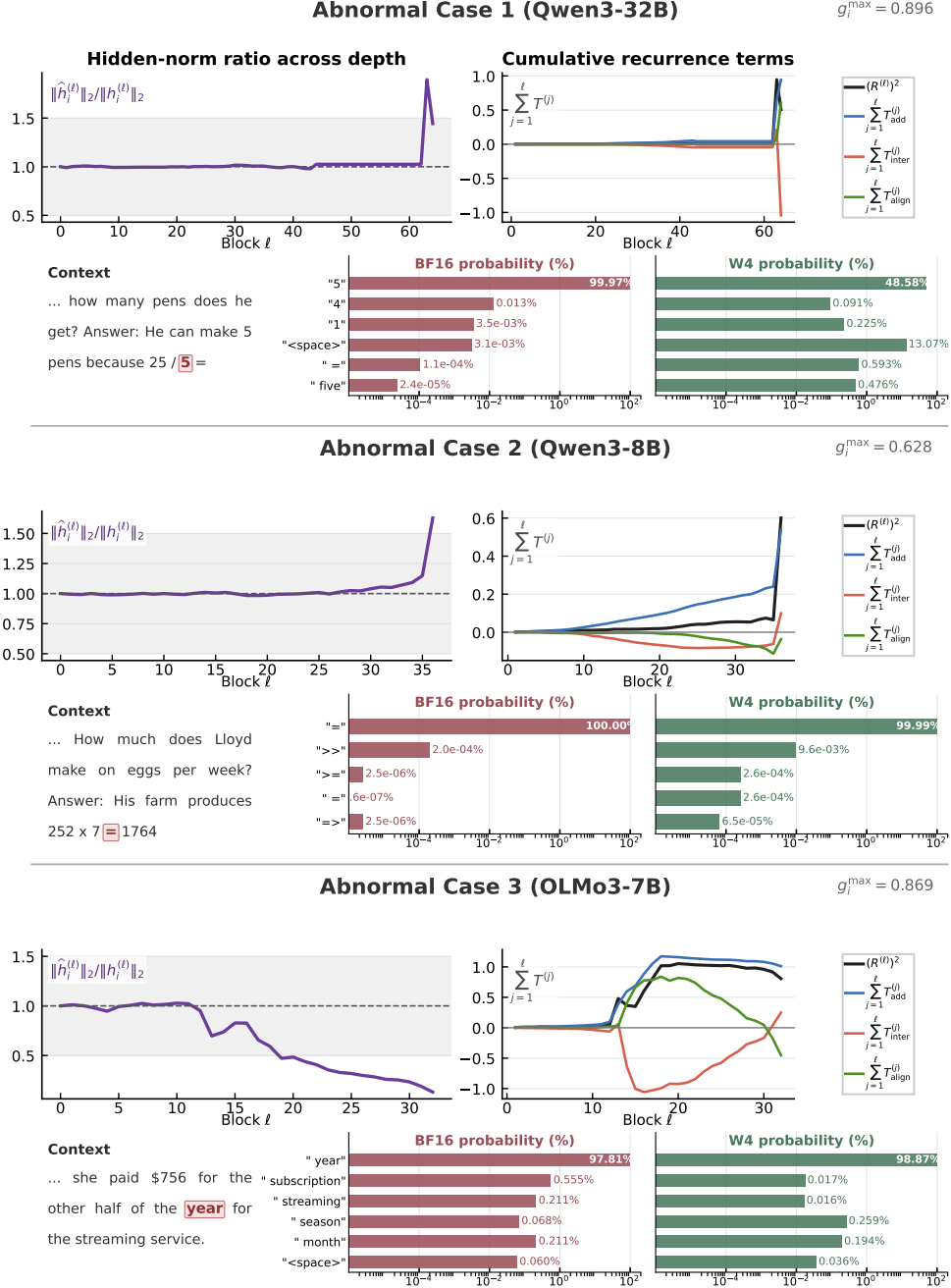
Figure 12: Rare hidden-state trajectory failures occur when BF16 and W4 hidden norms diverge. All three cases are from GSM8K text. Rows show Qwen3-32B, Qwen3-8B, and OLMo3-7B positions selected by proximity to each model’s median excluded g_i^{\max} ; the value beside each row title is this selection statistic, not the plotted ordinate. Selection does not use recurrence values or output changes. The left column shows \|\hat{\mathbf{h}}_i^{(\ell)}\|_2 / \|\mathbf{h}_i^{(\ell)}\|_2 , with the retained range [0.5, 1.5] shaded in gray. The right column shows the cumulative recurrence terms. Both columns use decoder block \ell on the horizontal axis. The lower strip shows the context and BF16/W4 next-token probabilities.
