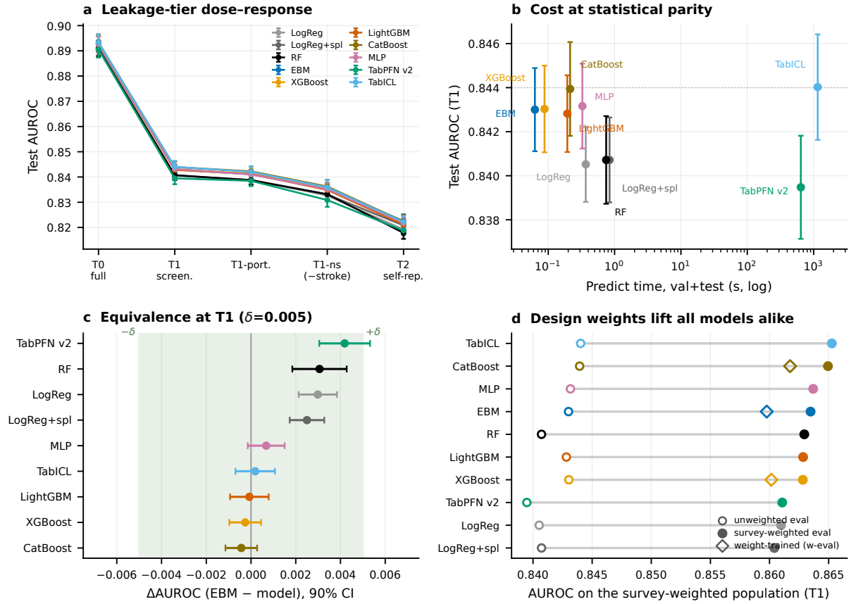
Figure 2. Leakage, cost, equivalence and design weights. (a) Test AUROC (mean \pm SD, five seeds) across leakage tiers, ordered by impact. (b) Accuracy versus prediction time on the validation and test workload, logarithmic scale. (c) Non-inferiority forest at T1: difference in AUROC (glass-box minus comparator) with 90% confidence intervals against the pre-specified \pm 0.005 band. (d) Survey design weights lift all models nearly uniformly; open diamonds denote weight-informed training.
