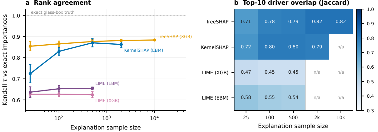
Figure 6. Post-hoc explanation is an estimate; glass-box explanation is an identity. (a) Kendall \tau between post-hoc attributions and the glass-box model’s exact global importances versus explanation sample size; LIME applied to the glass-box model itself plateaus at \tau \approx 0.63 , acquitting the cross-model confound while confirming the estimator limitation. (b) Overlap of each explainer’s ten strongest drivers with the exact top ten (Jaccard index); grey cells were not computed for tractability.
