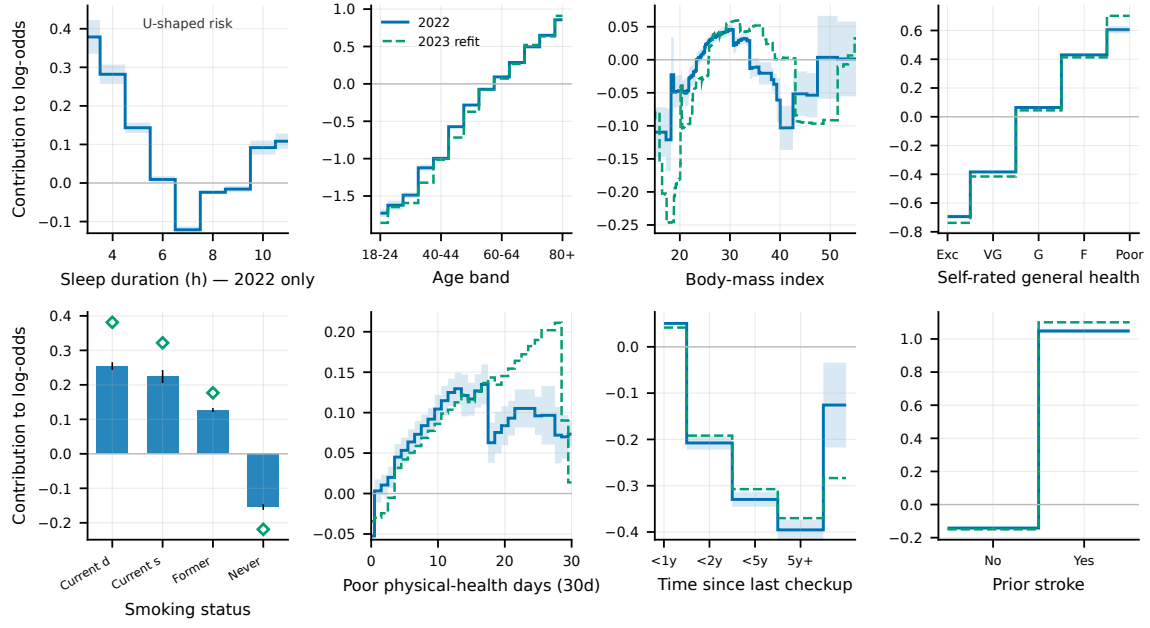
Supplementary Fig. 4 | Learned risk shapes and their replication across survey years. Glass-box term contributions for continuous, ordinal and categorical predictors: 2022 (with bagged uncertainty) versus an independent 2023 refit on the year-portable tier. Sleep duration was removed from the 2023 core questionnaire and is therefore shown for 2022 only.
