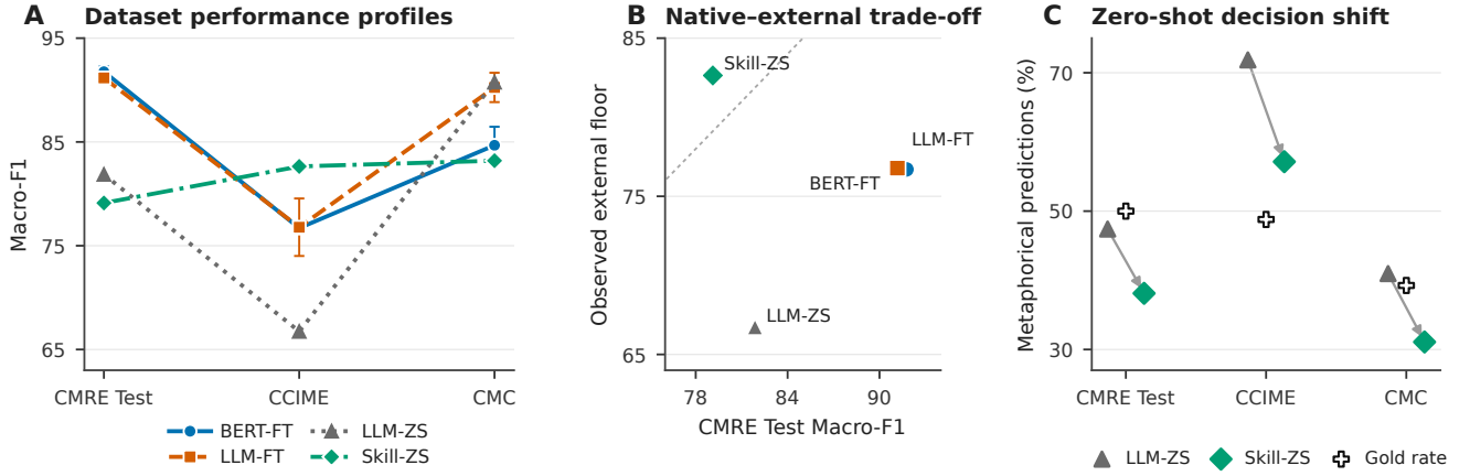
Fig. 1. Complementary profiles. (A) Macro-F1 by dataset. (B) CMRE Test Macro-F1 versus the observed external floor; the diagonal marks equality. (C) Rates of metaphorical predictions for the matched zero-shot pair and gold prevalence; arrows run from LLM-ZS to Skill-ZS. Whiskers show sample SD only for the three-seed fine-tuned conditions.
