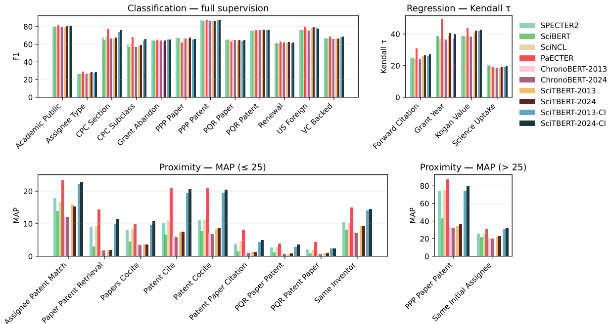
Figure 2: Performance of 2013 and 2024 vintage SciTBERT and SciTBERT-CI models, alongside a number of prior encoder models, across a selection of PatRepEval tasks.
