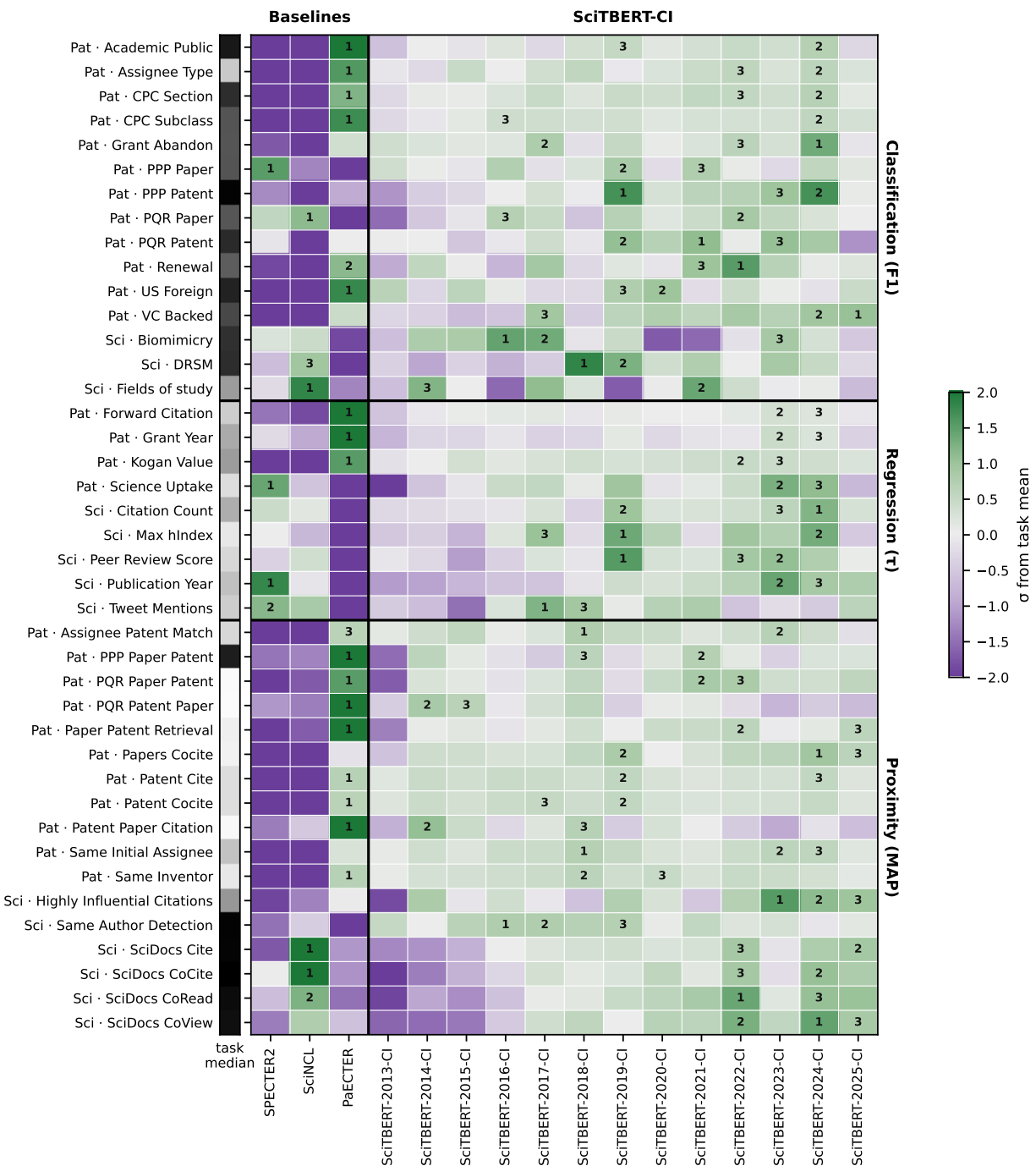
Figure 6: Relative performance of SciTBERT-CI models versus similar contrastively post-trained scientific models. Performance is reported in standard deviations from the task mean performance across the models. The first-, second-, and third-best performing model for the task is denoted with a 1, 2, or 3, respectively.
