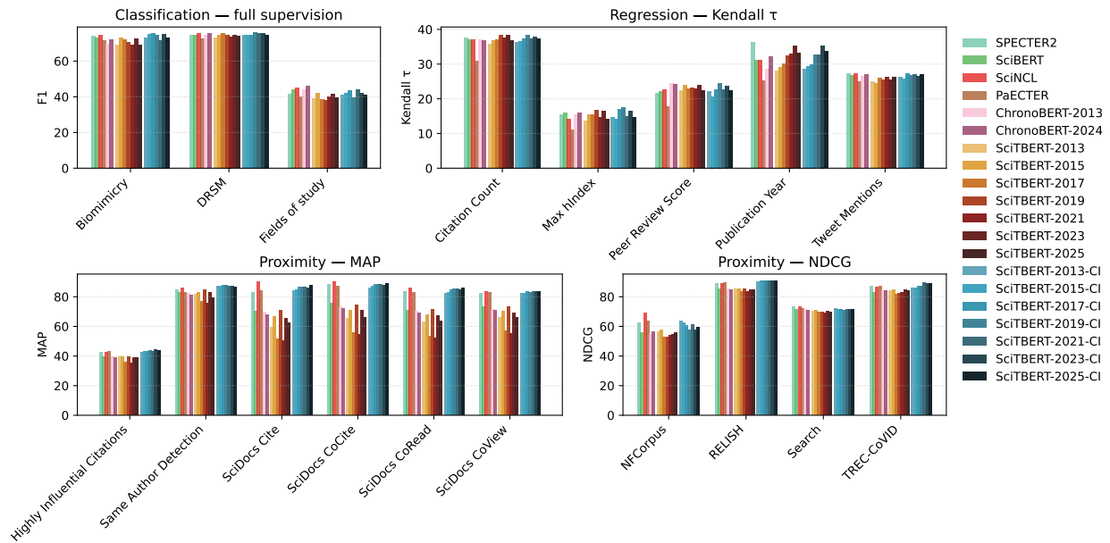
Figure 3: Performance of odd-year SciTBERT and SciTBERT-CI models, alongside a number of baseline models, across a selection of SciRepEval tasks.
