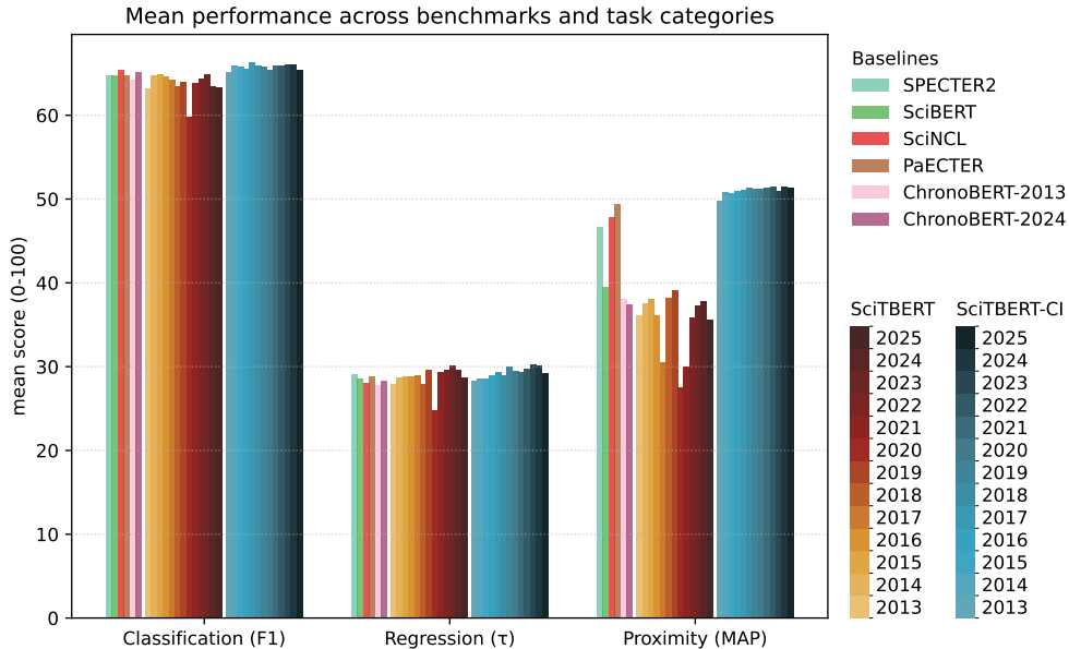
Figure 1: Performance of SciTBERT and SciTBERT-CI models, alongside a number of prior encoder models, across both SciRepEval and PatRepEval benchmarks. Performance is aggregated by taking the mean over the tasks of each category within each benchmark, then the mean of the two benchmarks. See Table 2.
