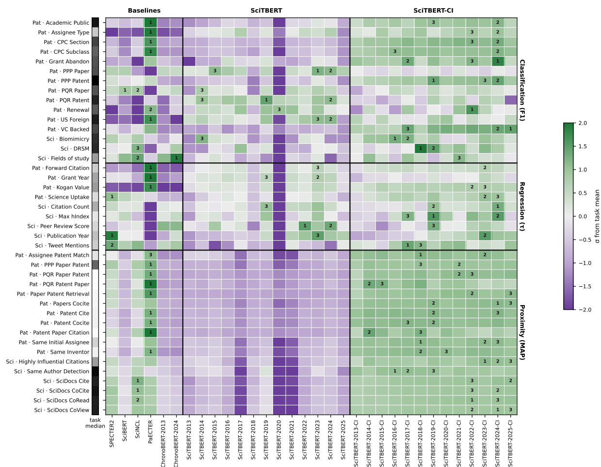
Figure 4: Relative performance of SciTBERT and SciTBERT-CI models versus similar scientific and chronologically timestamped models on all PatRepEval and SciRepEval tasks. Pat indicates PatRepEval tasks and Sci indicates SciRepEval tasks. Performance is reported in standard deviations from the task mean performance across the models. The first-, second-, and third-best performing model for the task is denoted with a 1, 2, or 3, respectively.
