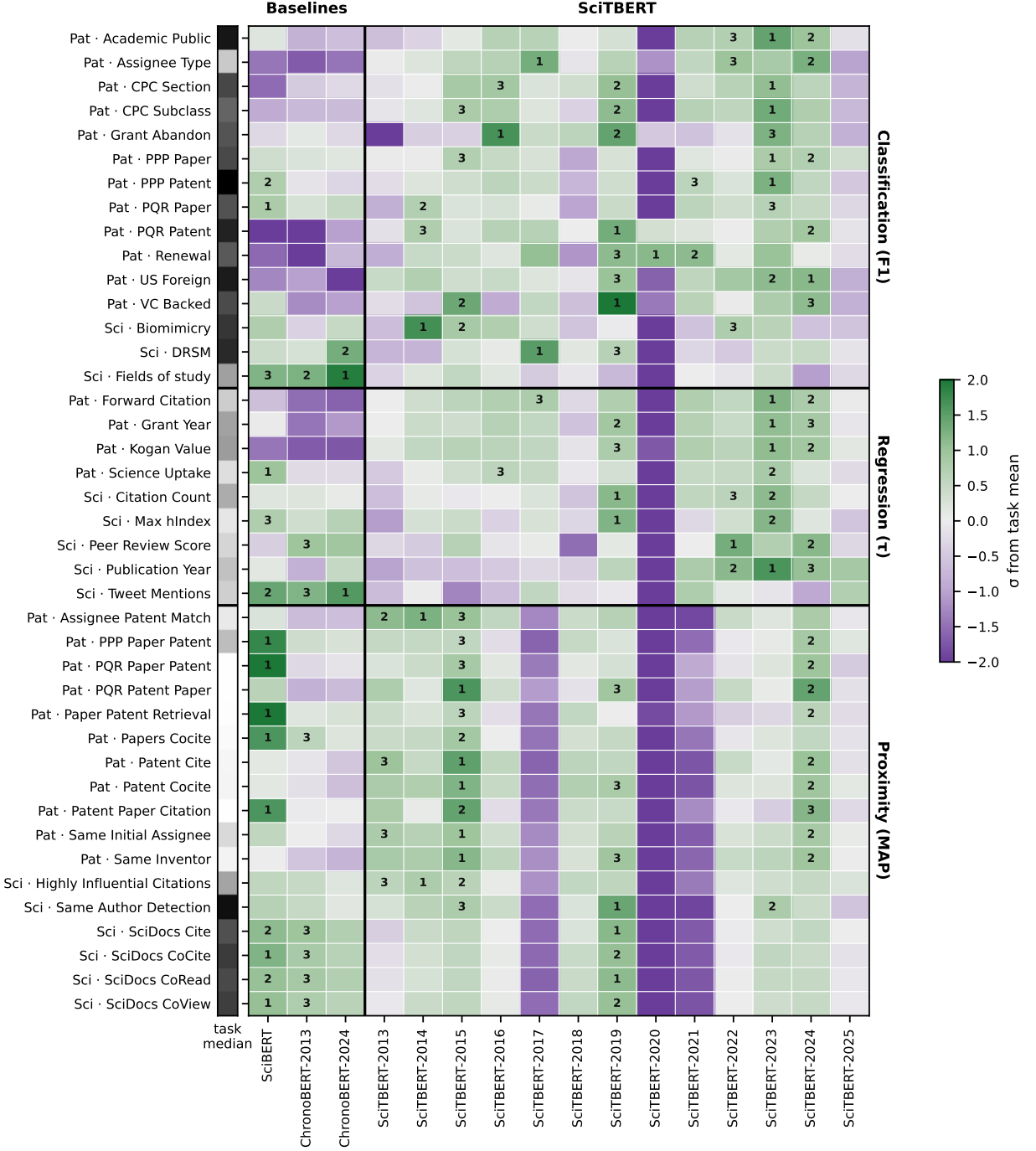
Figure 5: Relative performance of SciTBERT models versus baseline MLM-only scientific and timestamped models across both benchmark tasks. Performance is reported in standard deviations from the task mean performance across the models. The first-, second-, and third-best performing model for the task is denoted with a 1, 2, or 3, respectively.
