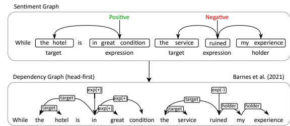
Figure 1: Head-first transformation of a sentiment graph to a dependency graph [5]. The sentiment graph has two opinion tuples: O_1 = (\emptyset, \text{the hotel}, \text{in great condition}, +) and O_2 = (\text{my experience}, \text{the service}, \text{ruined}, -) .
