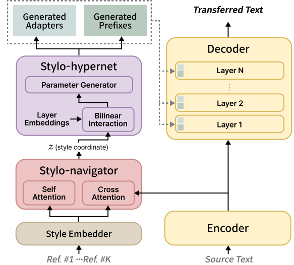
Figure 1: Overall architecture of HyperStyler
