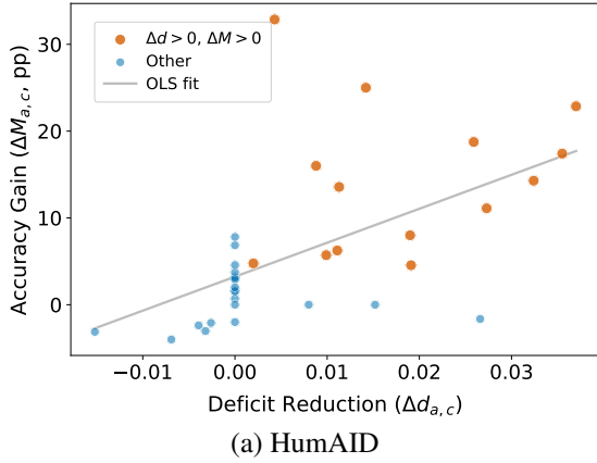
Figure 6: Additional subgroup-label accuracy gain versus deficit reduction on HumAID and HateXplain.
