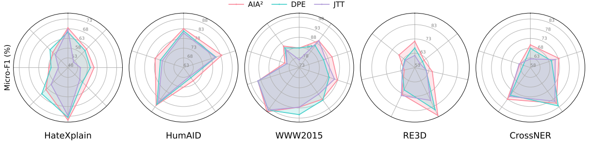
Figure 3: Subgroup-level Micro-F1 (%) across five datasets. Each radar plot compares AIA 2 with two representative baselines, JTT and DPE. Each spoke denotes a subgroup, and radial values indicate Micro-F1.
