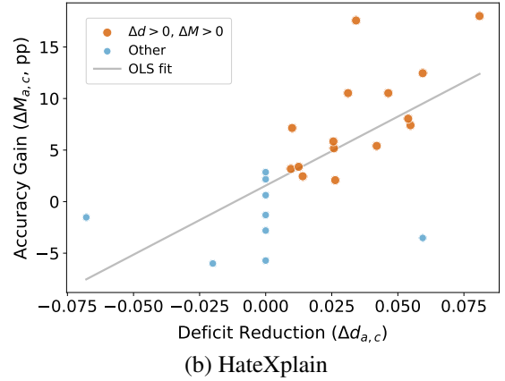
Figure 6: Additional subgroup-label accuracy gain versus deficit reduction on HumAID and HateXplain.
