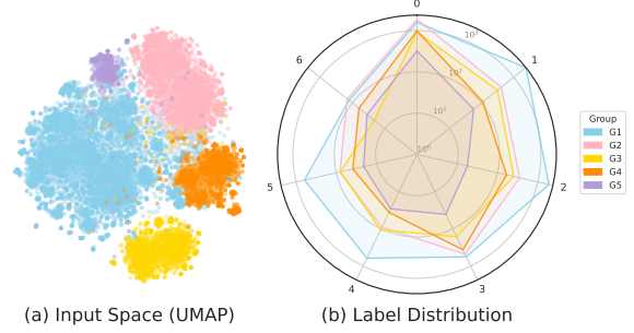
Figure 1: Subgroup-level distribution shifts in HumAID across different event sources (colors).
