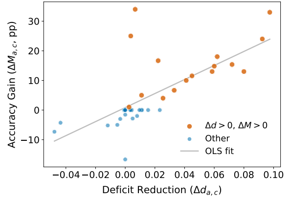
Figure 4: Subgroup-label accuracy gain versus deficit reduction on WWW2015, with an OLS fit.
