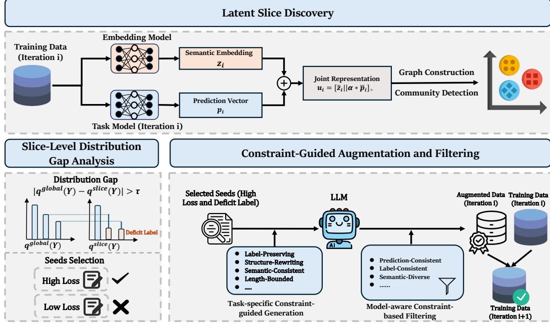
Figure 2: Overview of the AIA 2 framework. (1) Latent Slice Discovery partitions examples into coherent slices using joint semantic-predictive representations; (2) Slice-Level Distribution Gap Analysis identifies deficit labels and selects high-loss seeds; (3) Constraint-Guided Augmentation and Filtering generates and filters candidates for consistency and diversity. Augmented data is merged into the training set for the next iteration.
