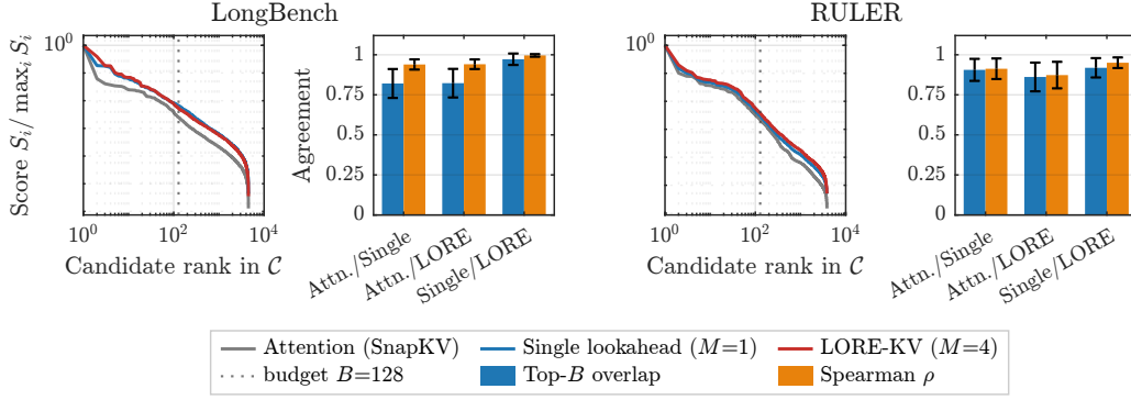
Figure 9: Retention-order shift. Candidate-score profiles, top- B overlap, and Spearman correlation across eviction criteria. Mistral-7B-Instruct-v0.2, B = 128 , M = 4 .
