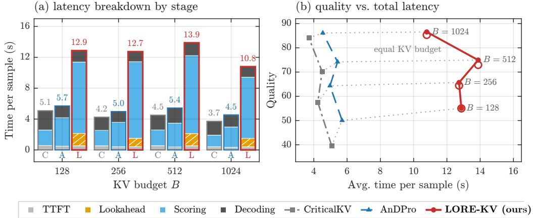
Figure 7: Latency-quality trade-off. (a) Stage-wise latency averaged over two seeds and (b) quality versus total latency across cache budgets on Mistral-7B-Instruct-v0.2, averaged over LongBench, RULER, and NIAH.
