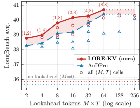
(b) Pareto frontier at matched lookahead-token budget
