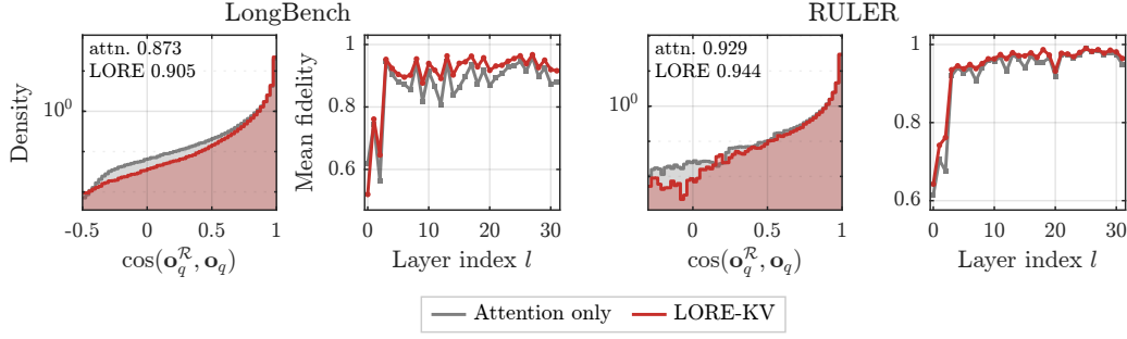
Figure 5: Attention-output fidelity. Similarity between retained- and full-cache outputs on future queries across layers. Mistral-7B-Instruct-v0.2, B = 128 .
