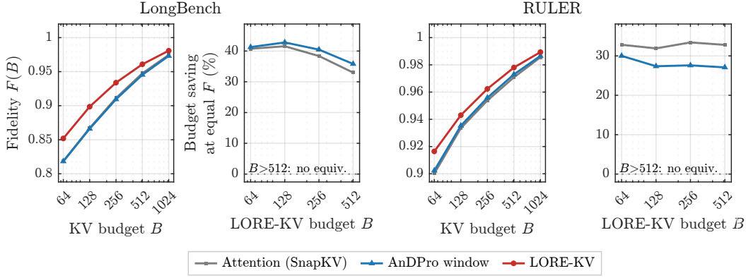
Figure 13: Budget equivalence under behavioral fidelity. Fidelity across cache budgets (left) and baseline cache savings required to match LORE-KV /E (right).
