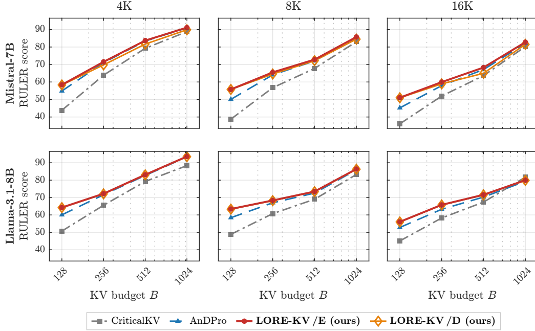
Figure 3: RULER accuracy averaged over 13 tasks at 4K, 8K, and 16K context lengths. Per-task results are given in Tables 7 and 10.
