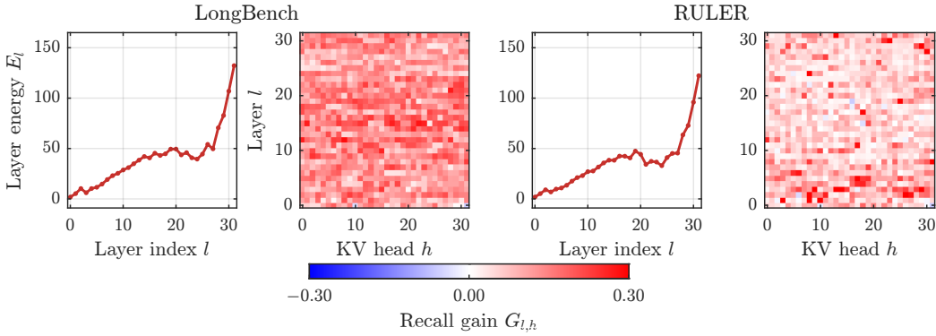
Figure 12: Future-query signal across layers and heads. Layer perturbation energy (left) and retention-recall gain from multi-lookahead queries (right). Mistral-7B-Instruct-v0.2, B = 128 , M = 4 .
