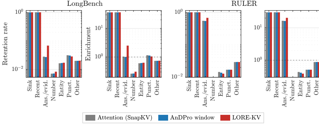
Figure 11: Retention by token class. Mean retained fraction (left) and class enrichment P(c | \mathcal{R})/P(c | X) (right).
