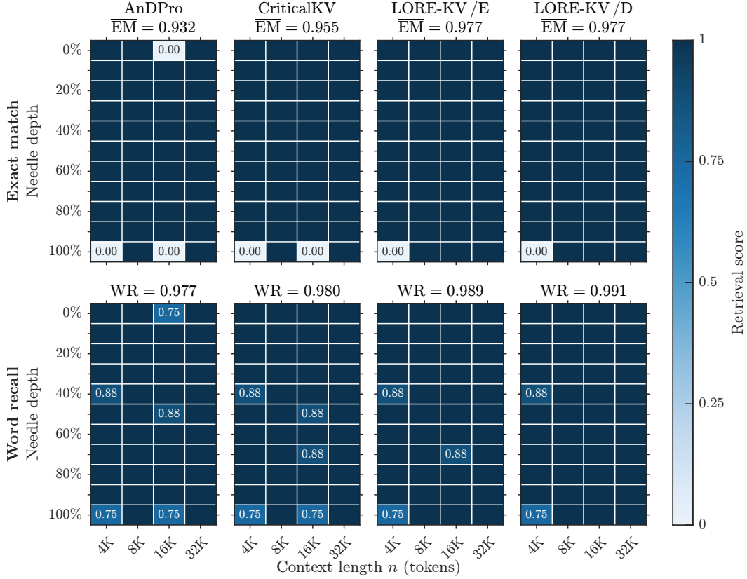
Figure 8: NIAH retrieval . Exact-match and word-recall scores across needle depths and 4K–32K contexts on Llama-3.1-8B-Instruct at B=1024 . Panel means are shown above each plot.
