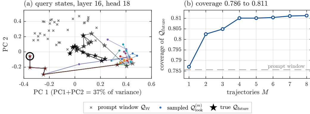
Figure 1: Monte Carlo future-query estimation: lookahead queries better match future decoding queries, with coverage saturating near M = 4 .
