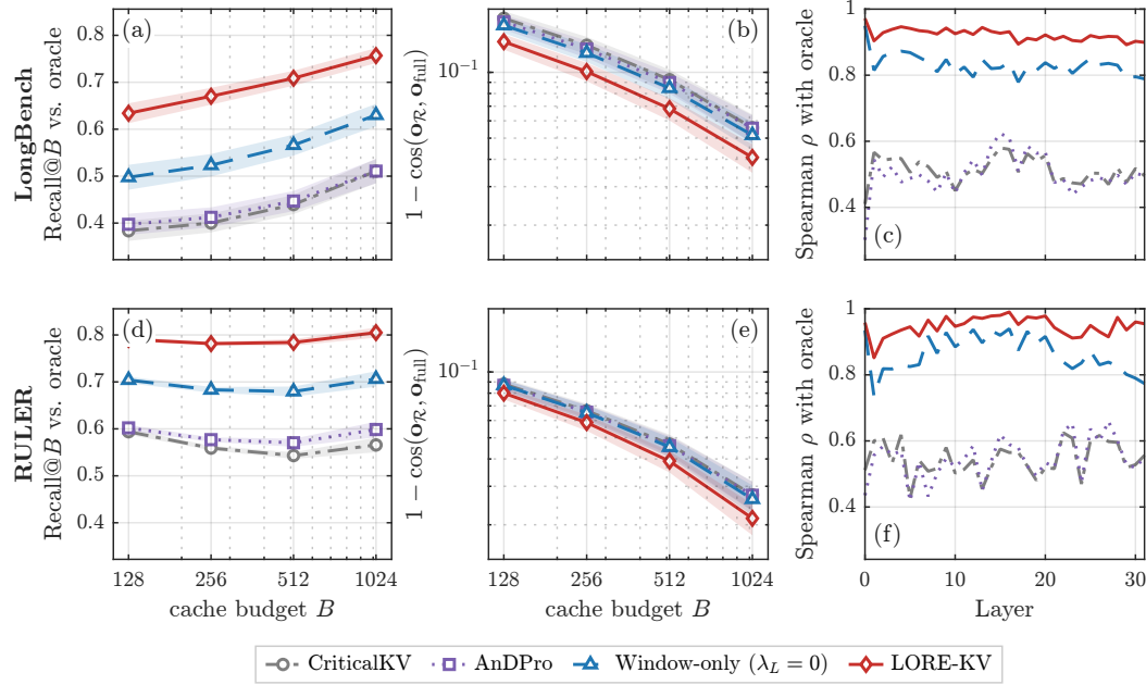
Figure 10: Criterion comparison. (a,d) Recall@ B against the future-query oracle. (b,e) Attention-output error (lower is better). (c,f) Layer-wise Spearman correlation with the oracle.
