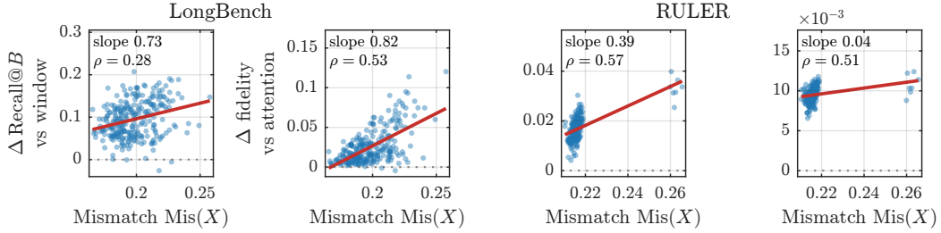
Figure 6: Gain versus query mismatch. Per-example gains in oracle retention and output fidelity with increasing prompt-to-future mismatch. Mistral-7B-Instruct-v0.2, B = 128 , M = 4 .
