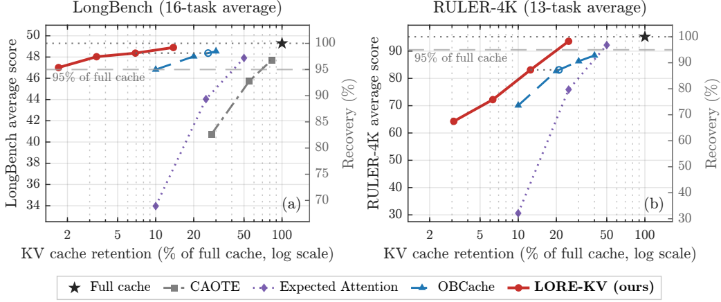
Figure 4: Accuracy-memory trade-off on Llama-3.1-8B-Instruct. Higher and further left indicates a better trade-off.
