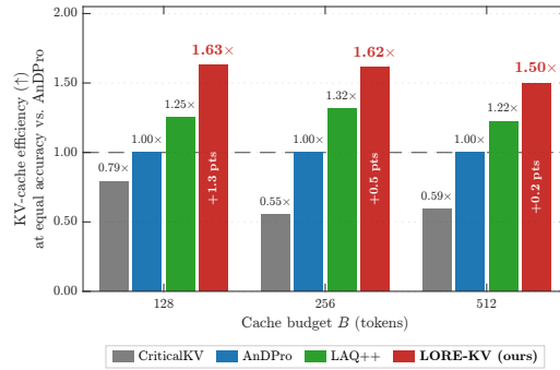
Figure 2: Equal-accuracy KV-cache efficiency on LongBench (Mistral-7B).
