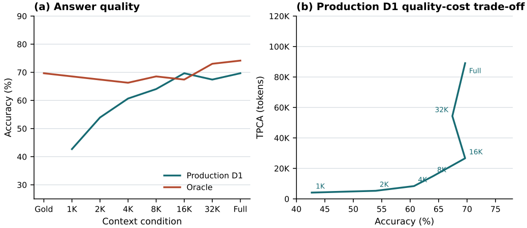
Figure 1: Main Accuracy by context-width condition for Production D1 and Oracle (left), and TPCA as a function of achieved Accuracy for Production D1 (right).
