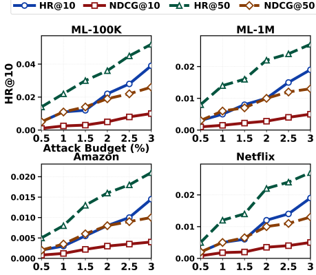
Fig. 11: Each panel reports performance as the injected fake-user budget grows: 0.5–3.0% of the user population.
