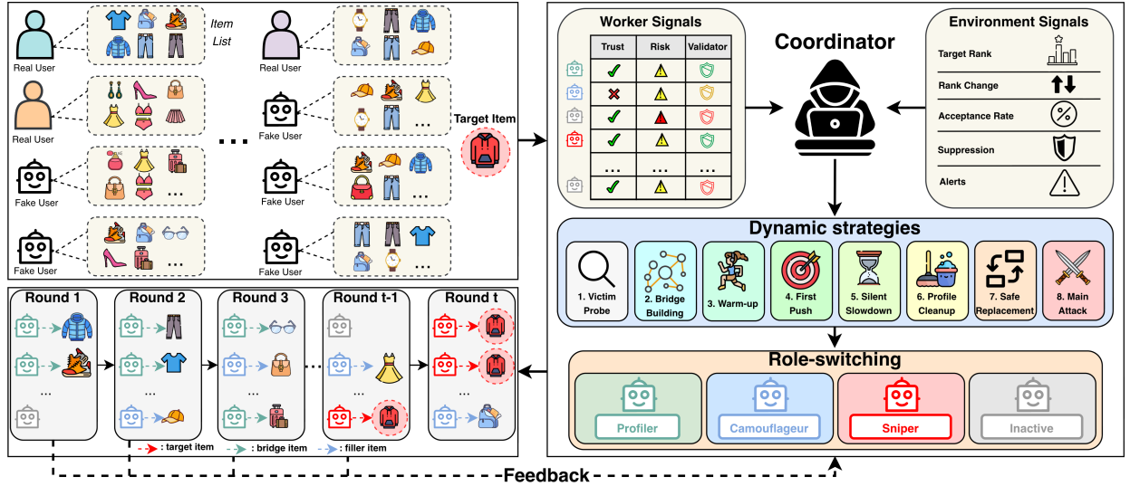
Fig. 2: Overview of the AGAS pipeline. Across attack rounds, the Coordinator aggregates worker and environment signals to adapt fake-user roles and attack strategies, progressively steering the campaign toward effective promotion of the target item. AGAS effectively uses feedback-derived signals to probe the victim, slow down when suppression emerges, and keep some workers inactive to avoid repetitive or overly synchronized behavior.
