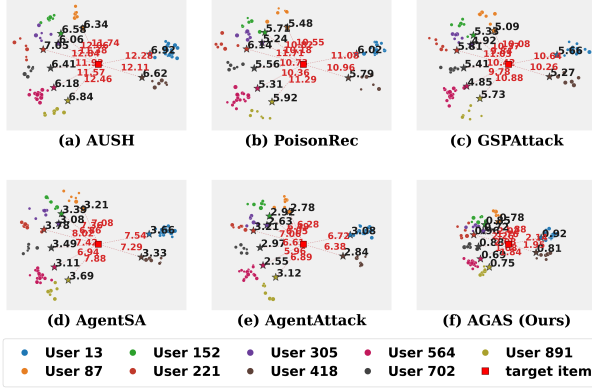
Fig. 3: t-SNE on ML-100K. Left : red = distance to target, black = distance to ground-truth items (smaller is stealthier). Right : clean (blue) vs. fake (star) user aggregate histories on poisoned victims. More scattered stars indicate better stealth.
