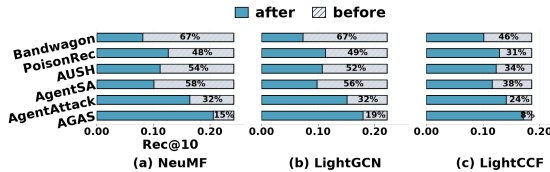
Fig. 5: Benign Rec@10 on three representative victims. The gray segment shows the gap to NoneAttack. Higher is better.
