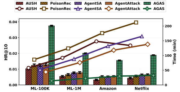
Fig. 9: Bars show HR@10 on the left axis, and lines show total runtime (minutes) on the right axis.
