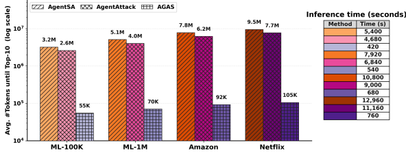
Fig. 10: Left : bar chart (log scale) of the average number of LLM tokens until the target first enters the Top-10. Right : the corresponding wall-clock seconds for each dataset.
