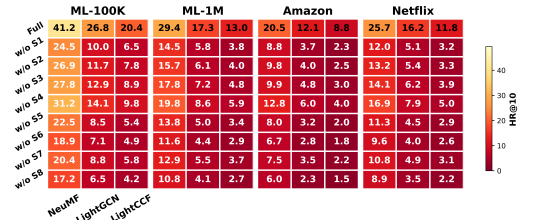
Fig. 6: Strategy ablation heatmap on four datasets. Columns correspond to three representative victims from MF, graph convolution, and graph contrastive families.
