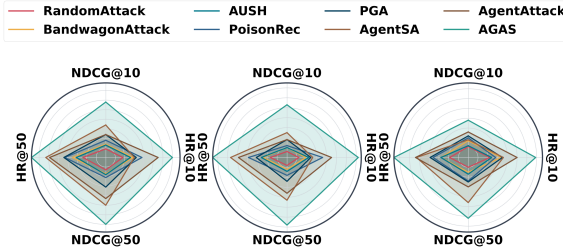
Fig. 4: Summary of Head/Mid attack performance across representative victims: GMF (MF), LightGCN (graph convolution), and XSimGCL (graph contrastive).
