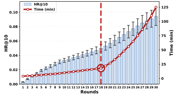
Fig. 8: Round-wise trade-off between HR@10 and runtime (minutes). Error bars show 95% CI.
