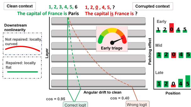
Figure 1: Overview of spontaneous context restoration. Patching effects shift across positions with depth, hidden states distinguish repaired from failed inputs, and early representations support failure triage before generation.
