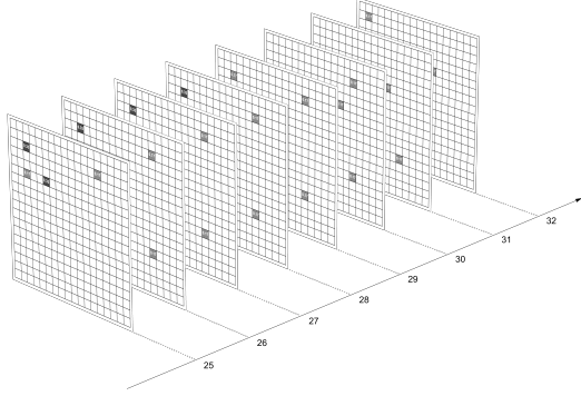
Figure 3: Eight successive matrices from the trajectory ( L = 6 , t = 25, \dots, 32 ). Darker cells indicate higher transition probability. With only five transitions per window, the support is sparse and changes whenever one transition enters or leaves.
