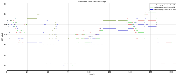
Figure 6: One illustrative draw for each L . Quantitative results are reported in Table 1; visual similarity is not used to select a window.
