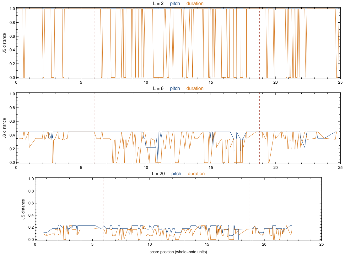
Figure 5: Successive transition-distribution JS distance between absolute-pitch and notated-duration transition distributions. Dashed lines mark the measure-9 and measure-26 references. A point on a high plateau is not an isolated boundary peak.
