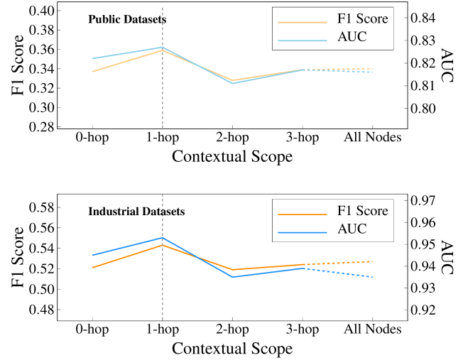
Figure 8: Performance vs. Contextual Scope ( k ) - RQ7.
