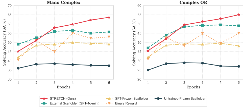
Figure 3: Ablation study on the necessity of difficulty alignment over a 6-epoch training on Learner by using the Qwen2.5-7B-Instruct backbone. We report Solving Accuracy (SA) on the Mano Complex (left) and Complex OR (right) datasets.
