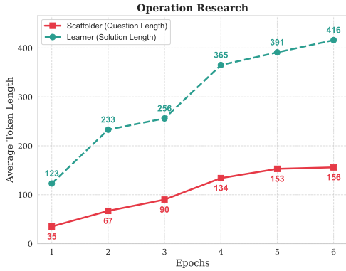
Figure 4: Quantitative co-evolution of question complexity (Scaffolder) and reasoning depth (Learner). The average token length of the generated questions and the successful reasoning trajectories exhibit a synchronized upward trend.
