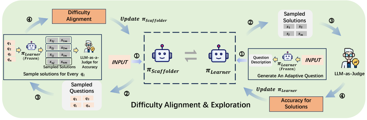
Figure 2: The dual-loop asynchronous updating mechanism of STRETCH. Difficulty Alignment (Left Loop): \pi_{Scaffolder} is updated to generate questions within the Learner’s Stretch Zone by driving a frozen Learner to sample solutions and evaluating its empirical accuracy. Exploration (Right Loop): \pi_{Learner} is updated to solve adaptive questions generated by a frozen Scaffolder.
