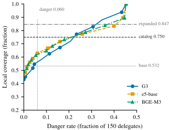
Figure 2: Both encoder gates hold more local coverage than the BM25-score gate throughout the danger budget. Reference lines mark the base rate and the two catalog ceilings.
