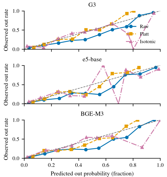
Figure 3: Calibration moves predicted probabilities toward the diagonal but does not change ranking. The staircase in the isotonic curves is an overfitting artifact of the finite calibration folds.
